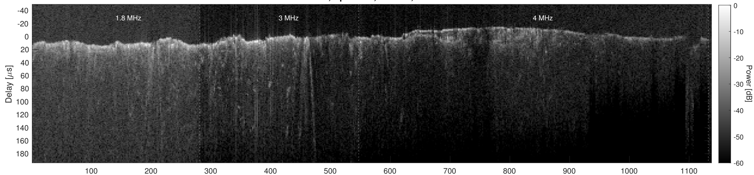
Orbit 4746, Cluttergram
