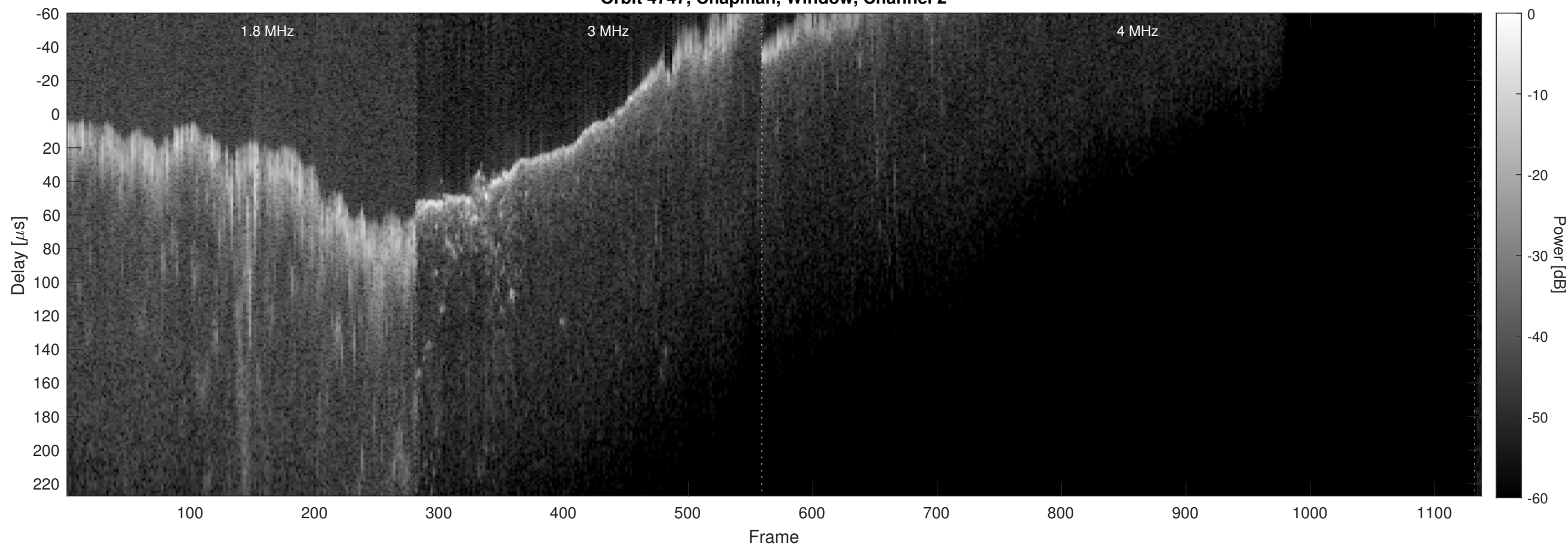
Orbit 4747, Chapman, Window, Channel 2
