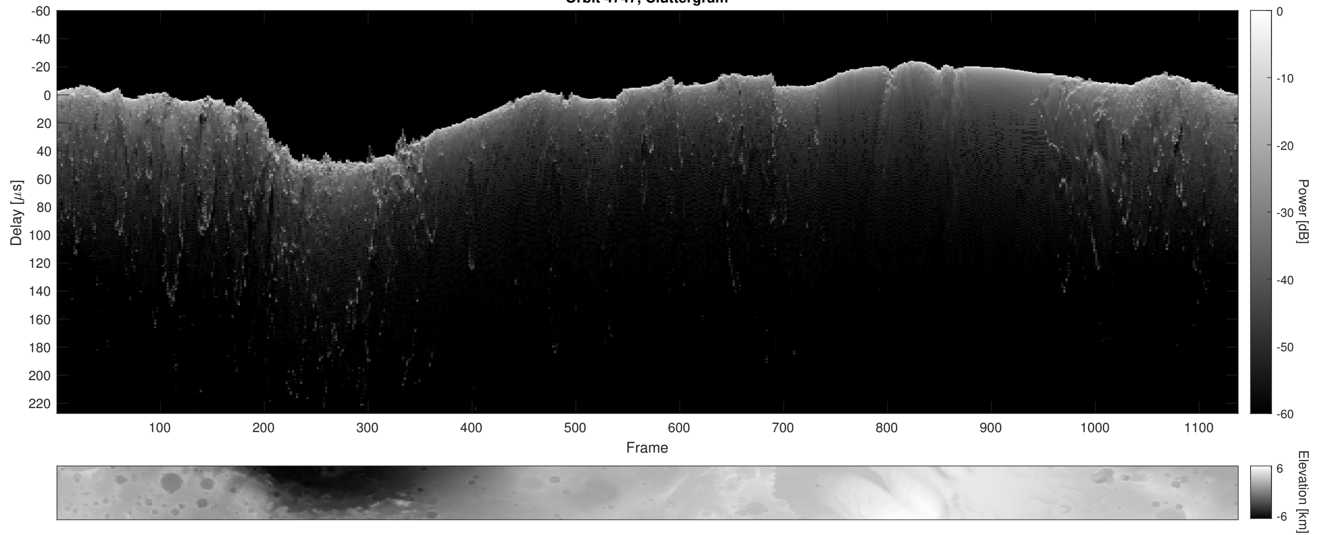
Orbit 4747, Cluttergram
