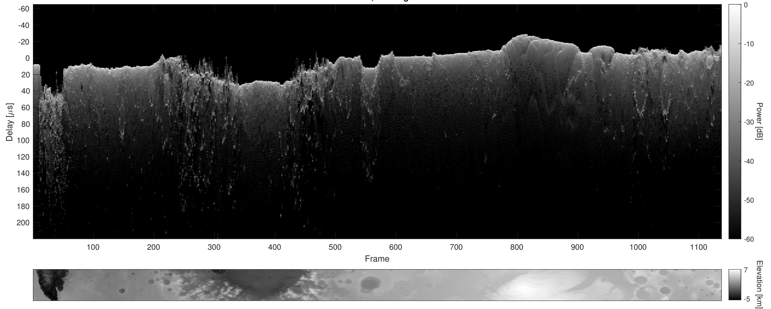
Orbit 4748, Cluttergram
