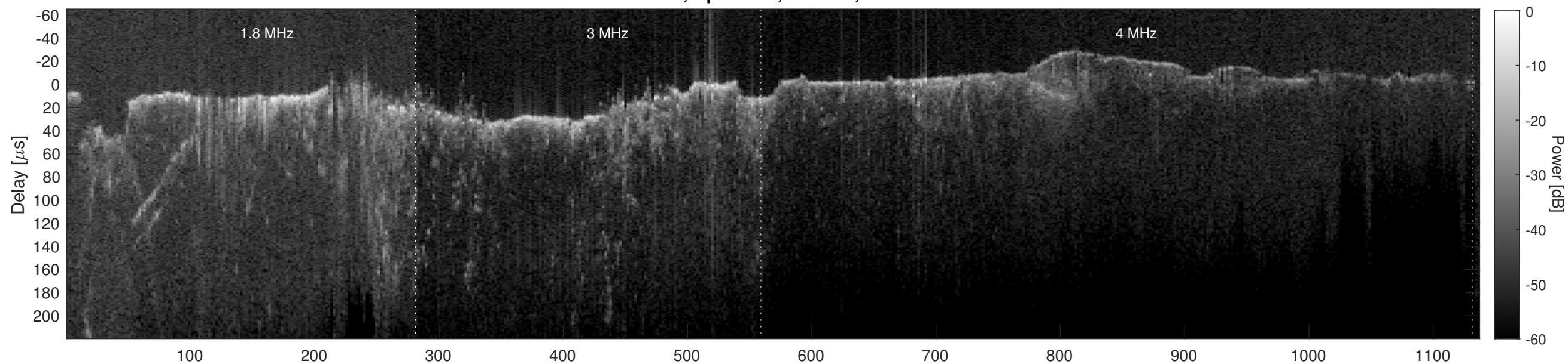
Orbit 4748, Cluttergram
