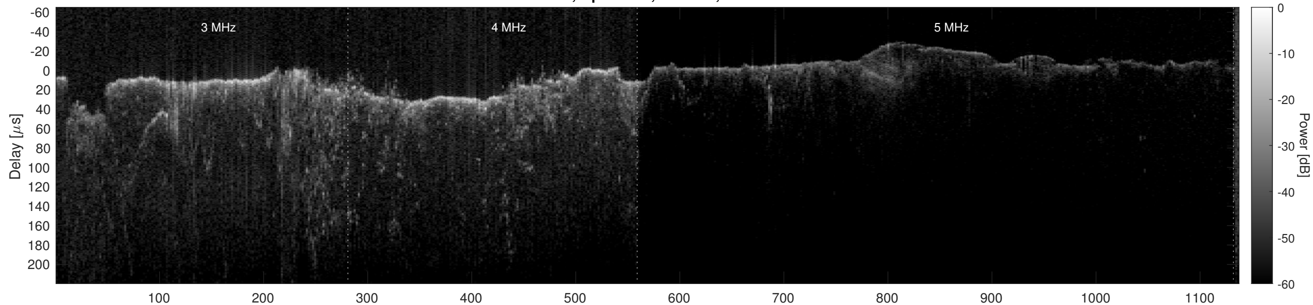
Orbit 4748, Optimized, Window, Channel 2
