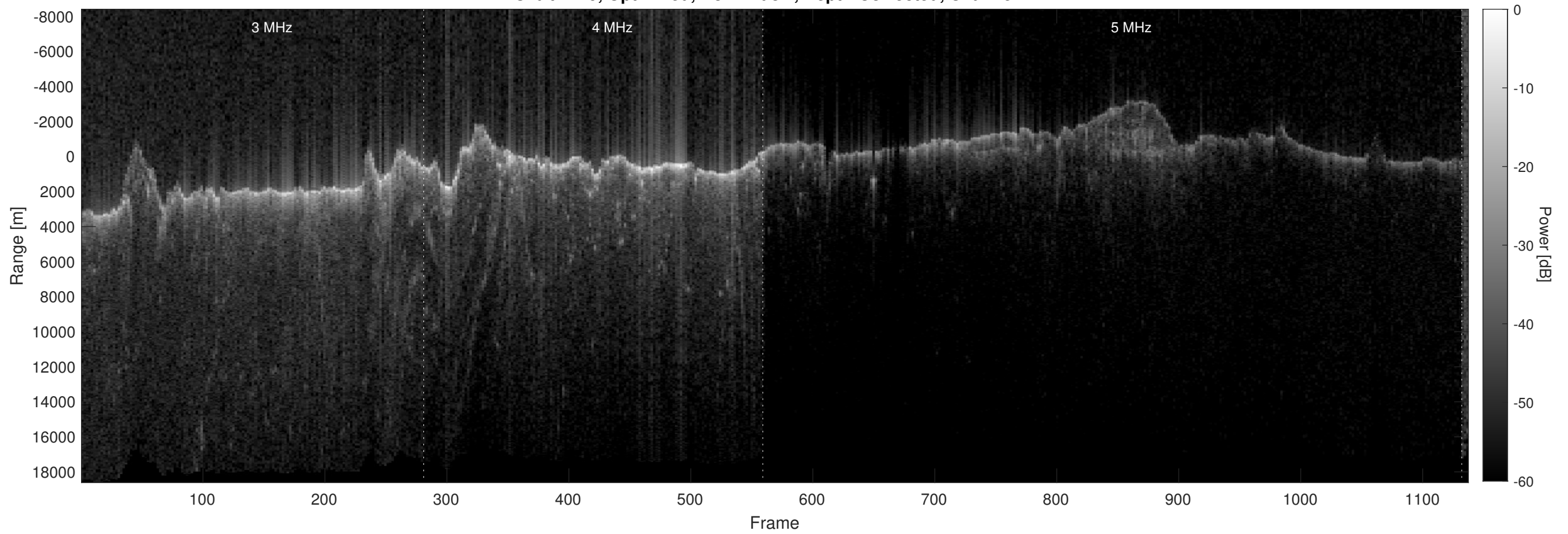
Orbit 4749, Optimized, No Window, Depth-Corrected, Channel 2
