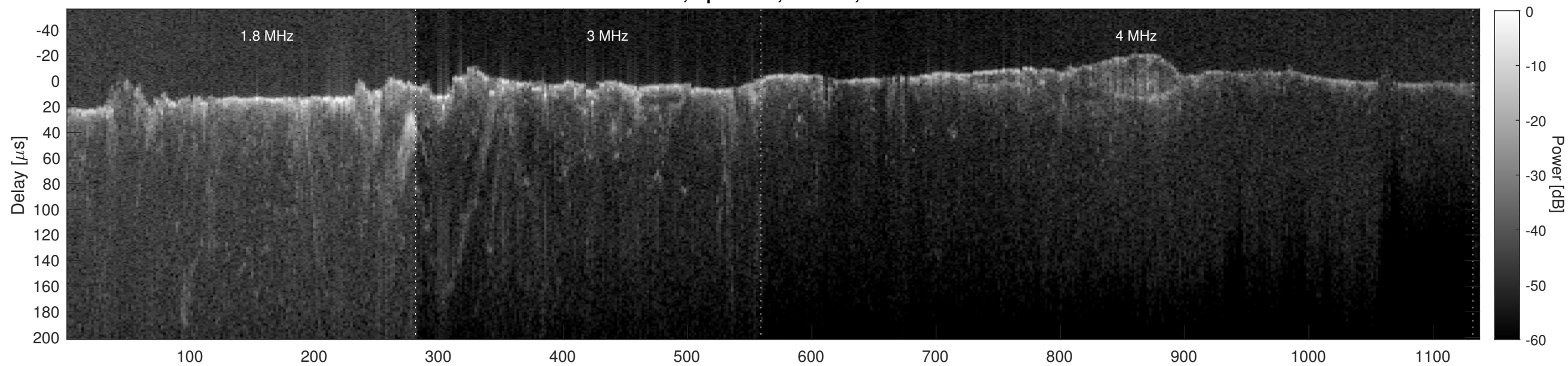
Orbit 4749, Cluttergram
