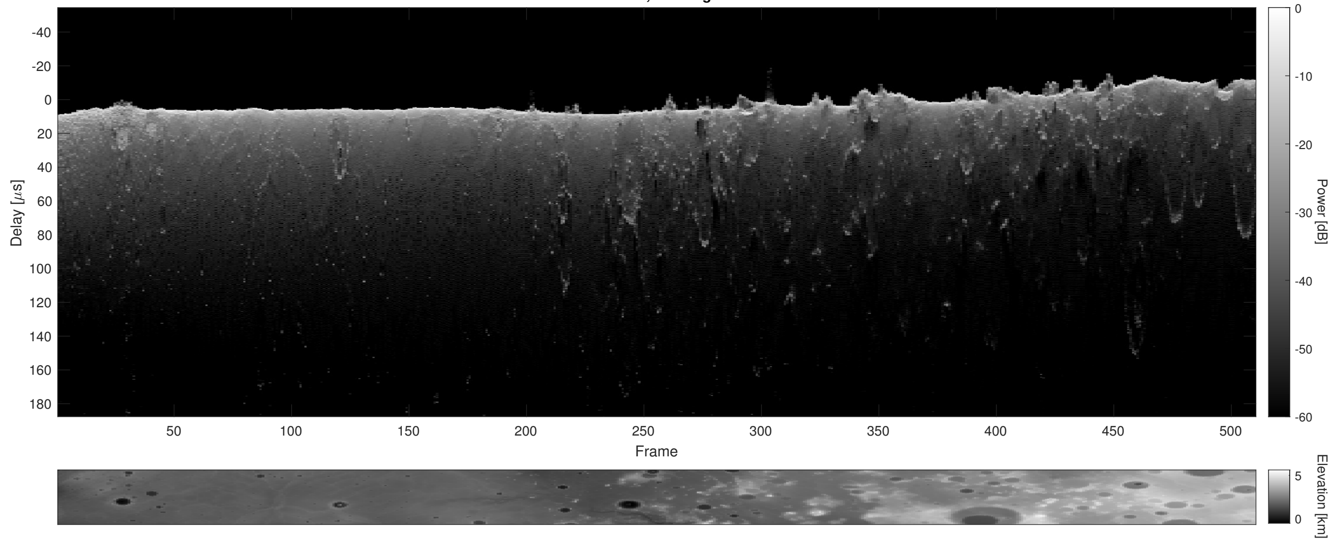
Orbit 4750, Cluttergram
