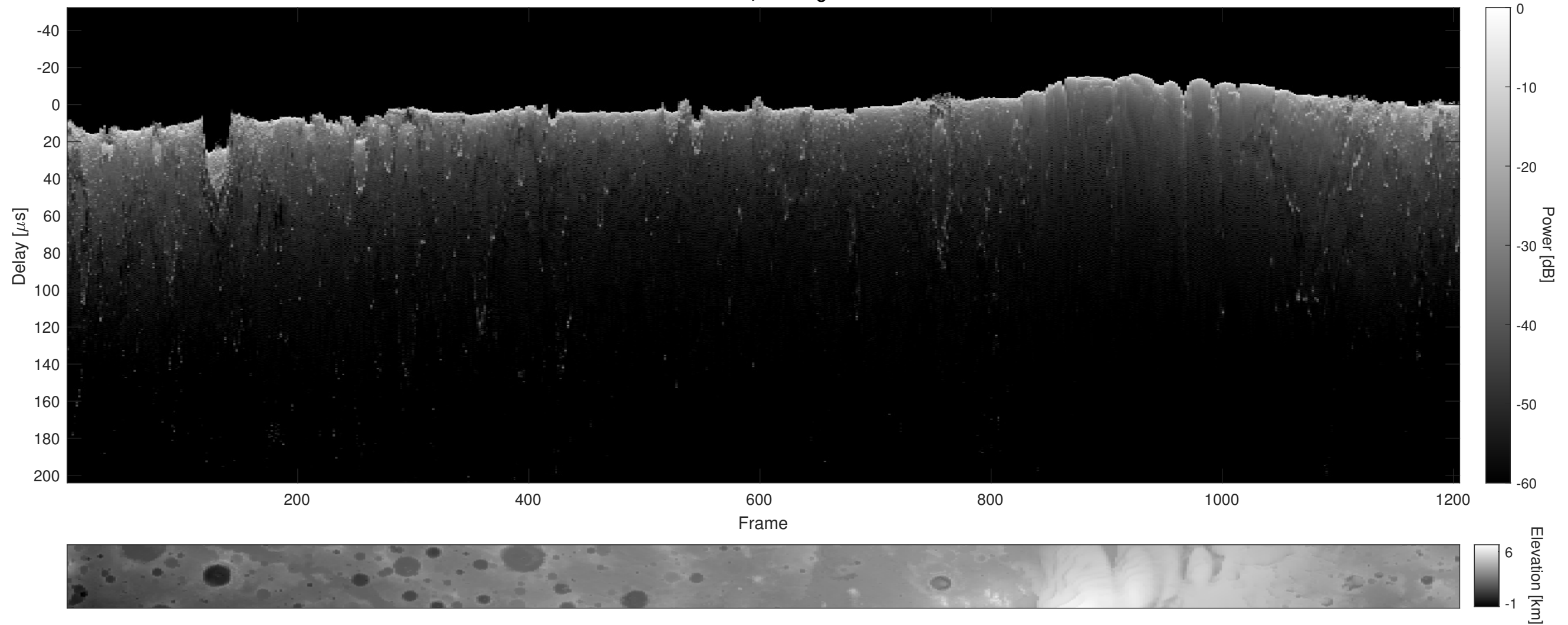
Orbit 4751, Cluttergram
