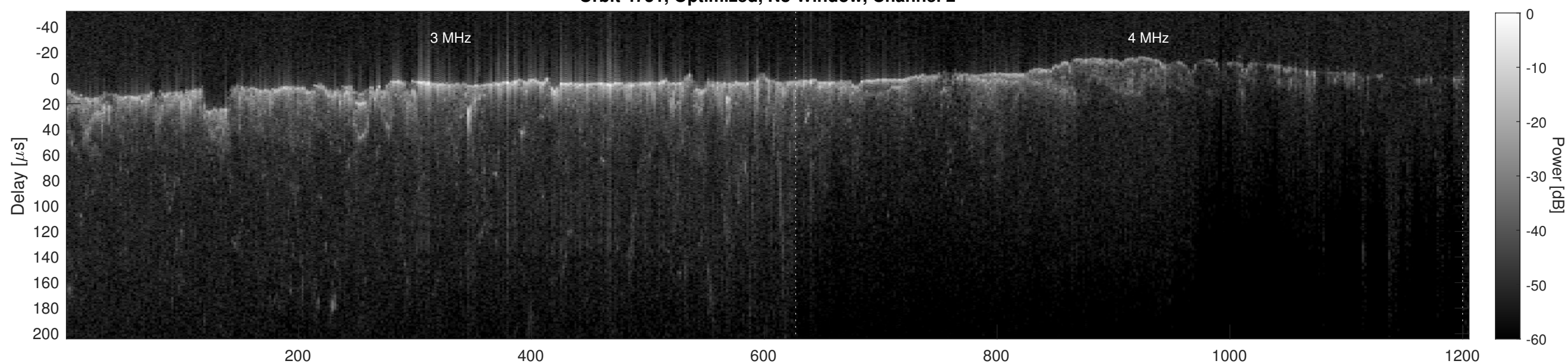
Orbit 4751, Cluttergram
