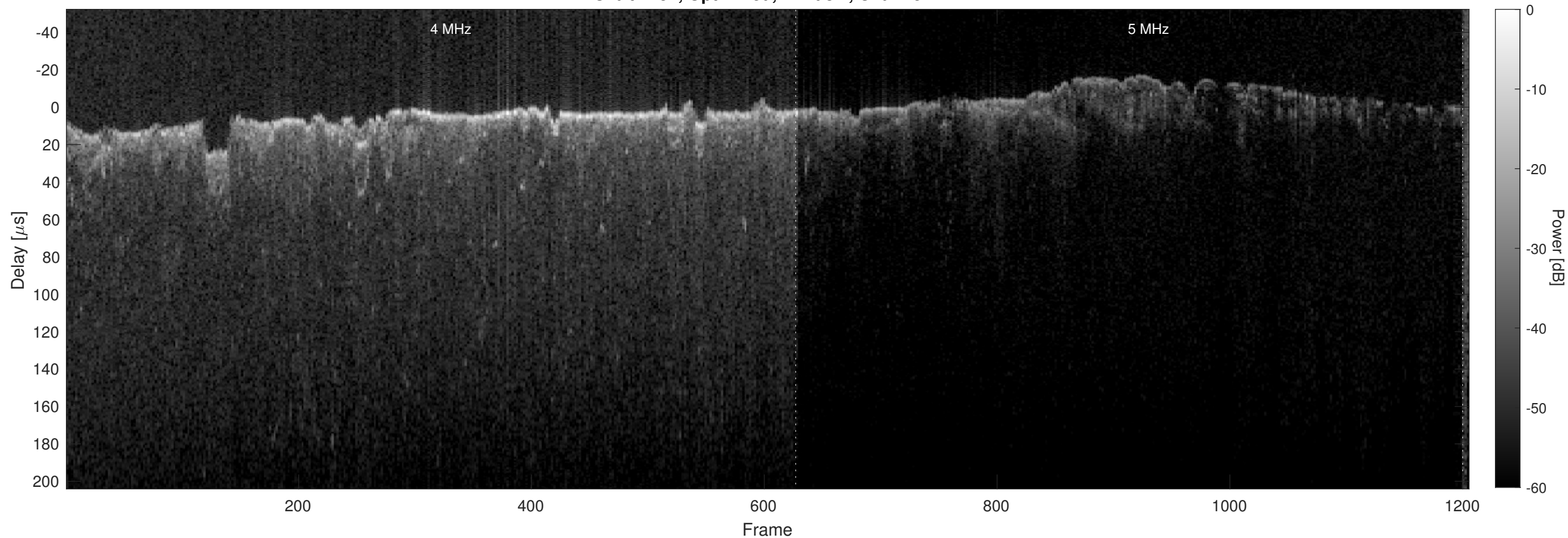
Orbit 4751, Optimized, Window, Channel 2
