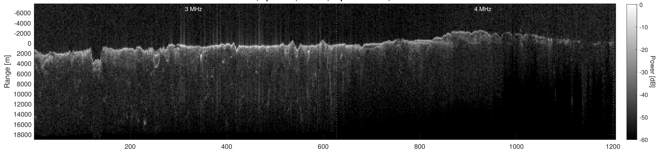
Orbit 4751, Depth-Corrected Cluttergram
