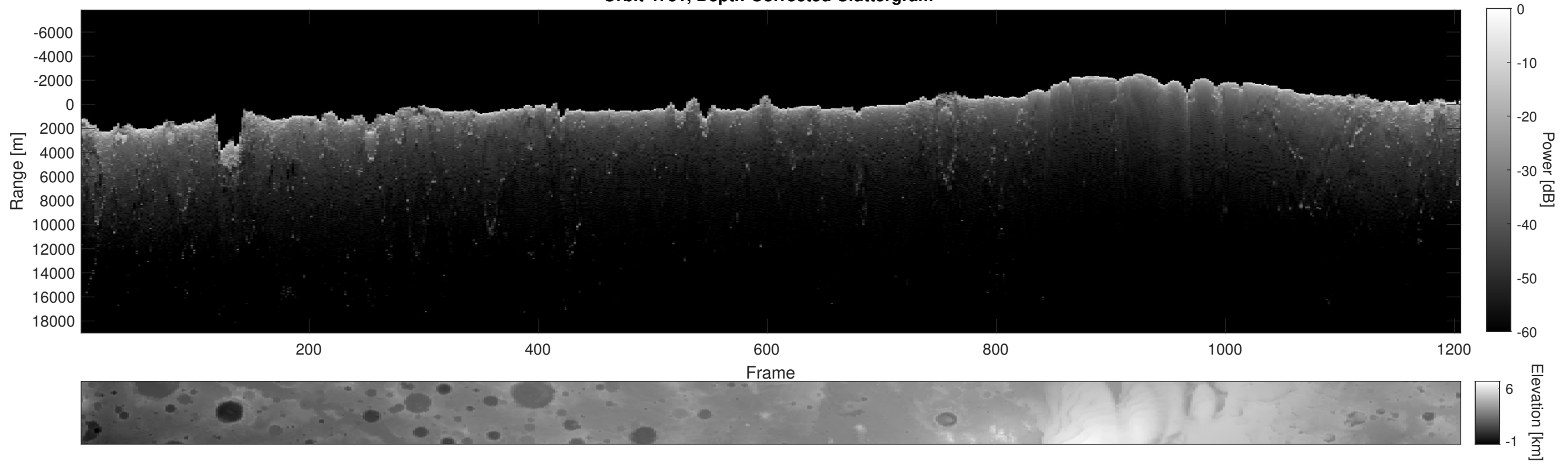
Orbit 4751, Depth-Corrected Cluttergram
