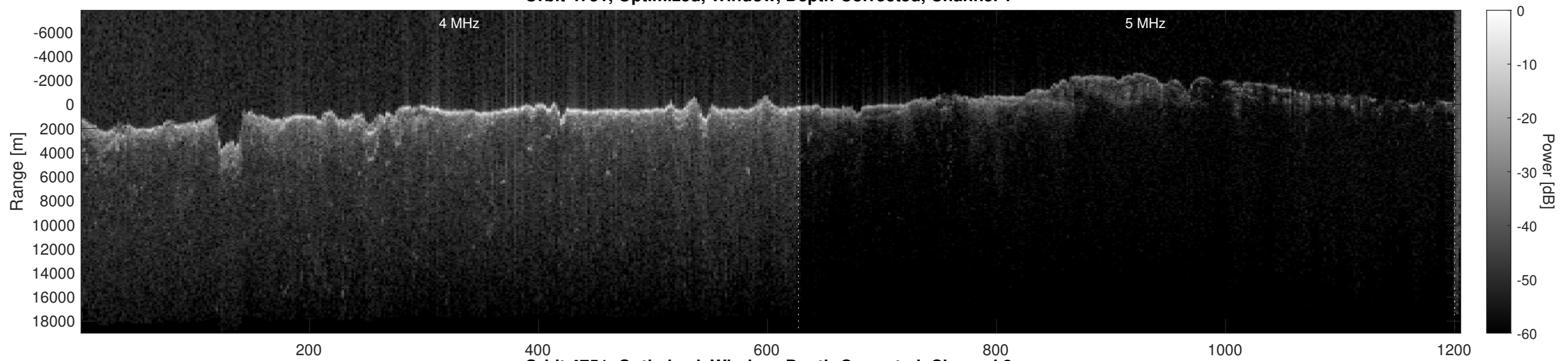
Orbit 4751, Optimized, Window, Depth-Corrected, Channel 2
