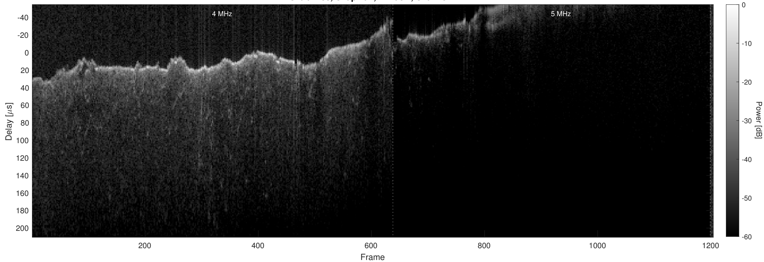
Orbit 4753, Chapman, Window, Channel 2
