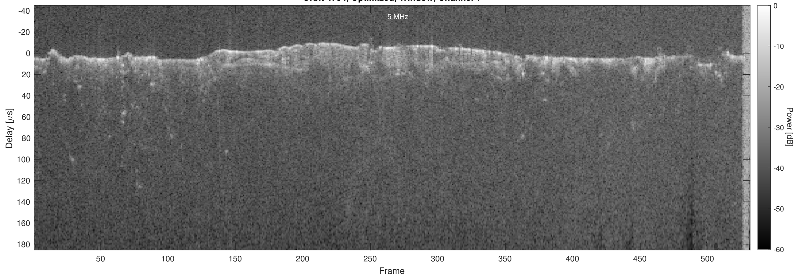
Orbit 4754, Optimized, Window, Channel 2
