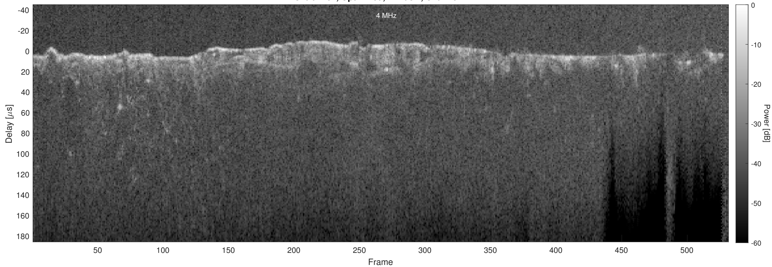
Orbit 4754, Optimized, Window, Channel 2
