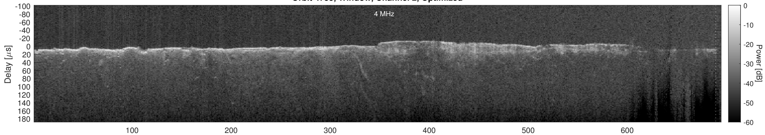
Orbit 4755, Cluttergram
