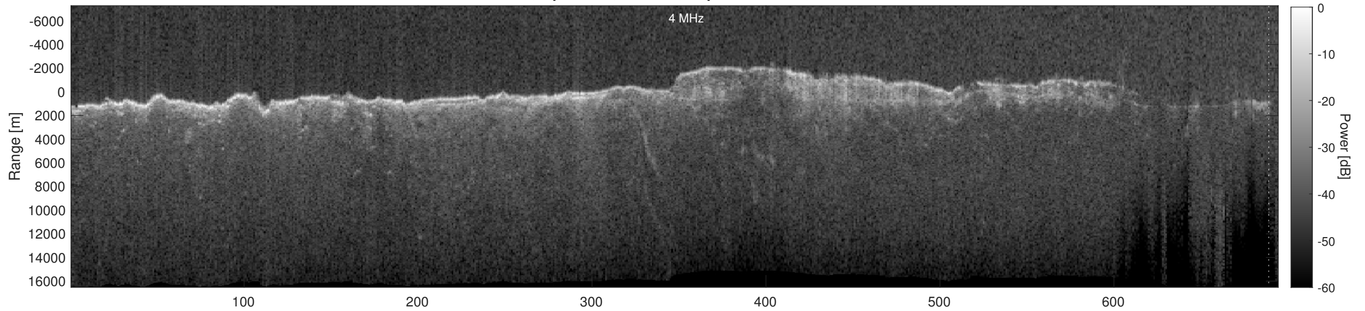
Orbit 4755, Depth-Corrected Cluttergram
