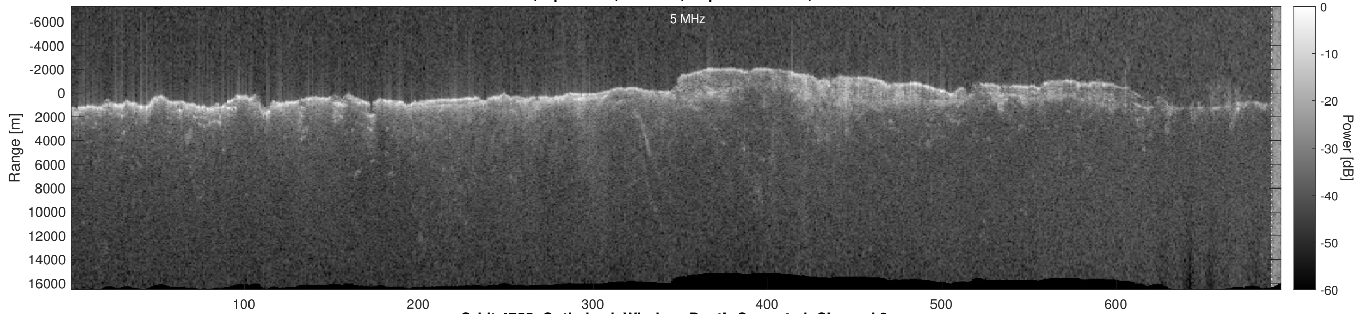
Orbit 4755, Optimized, Window, Depth-Corrected, Channel 2
