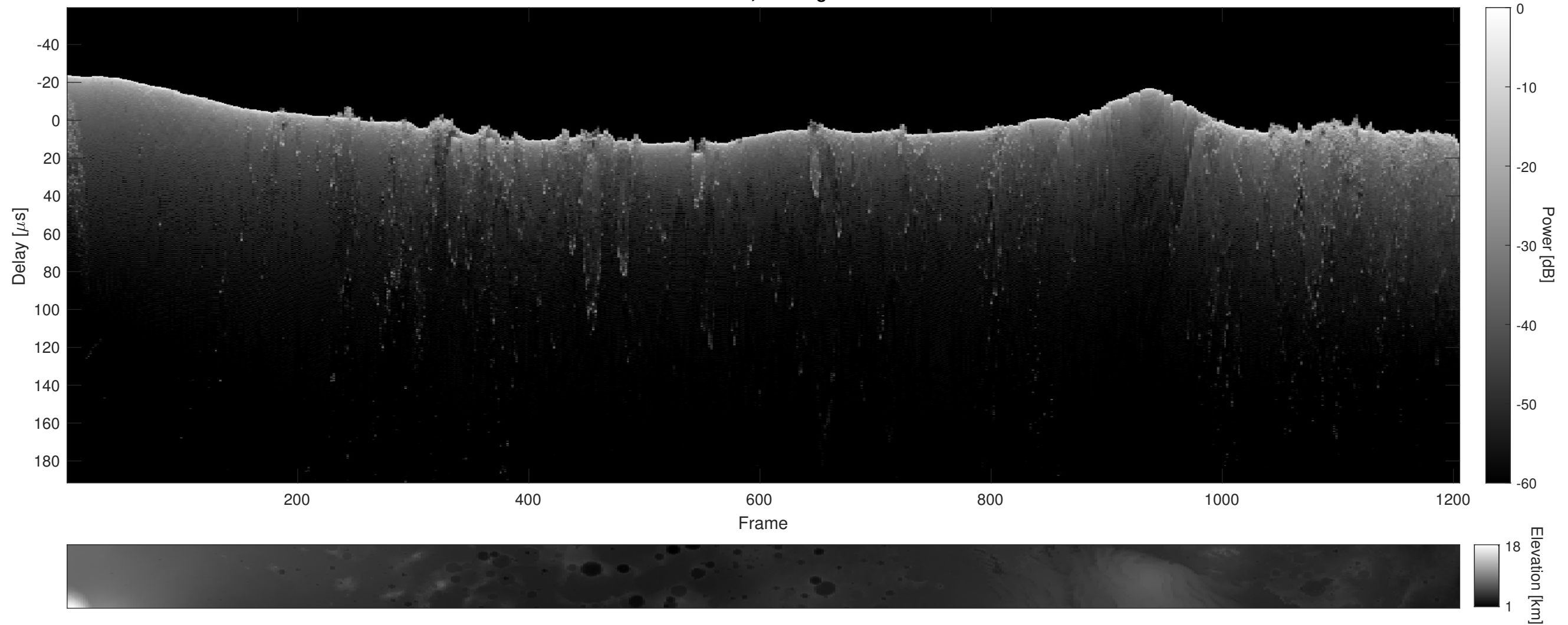
Orbit 4756, Cluttergram
