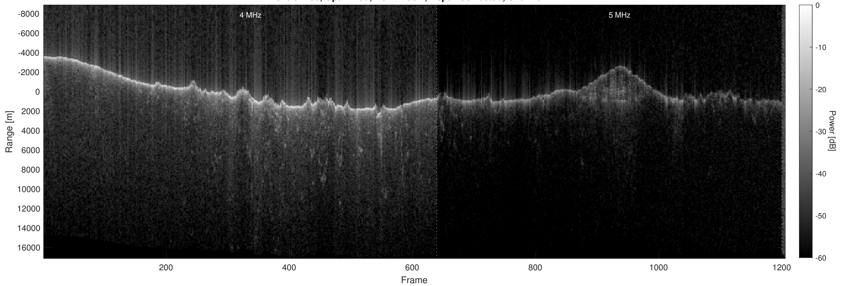
Orbit 4756, Optimized, No Window, Depth-Corrected, Channel 2
