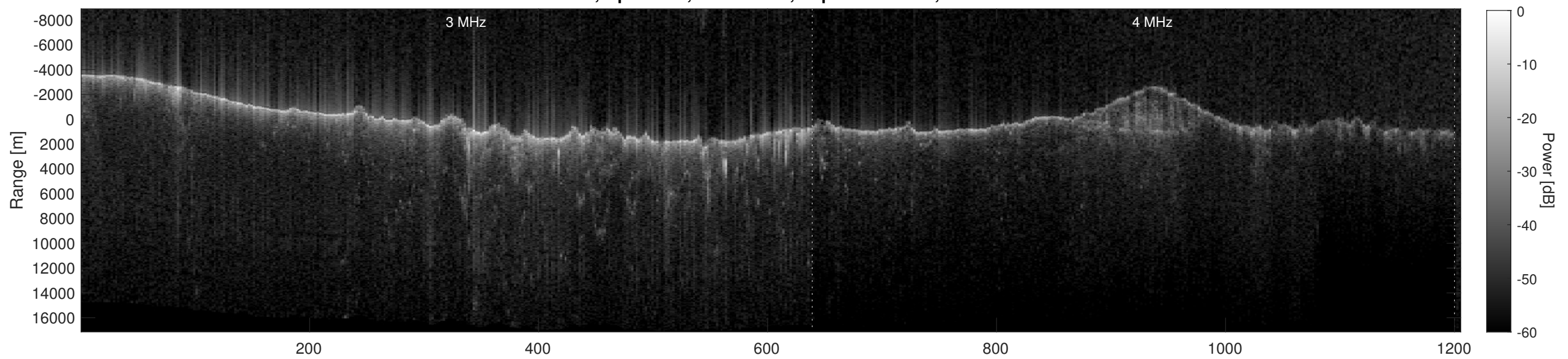
Orbit 4756, Depth-Corrected Cluttergram
