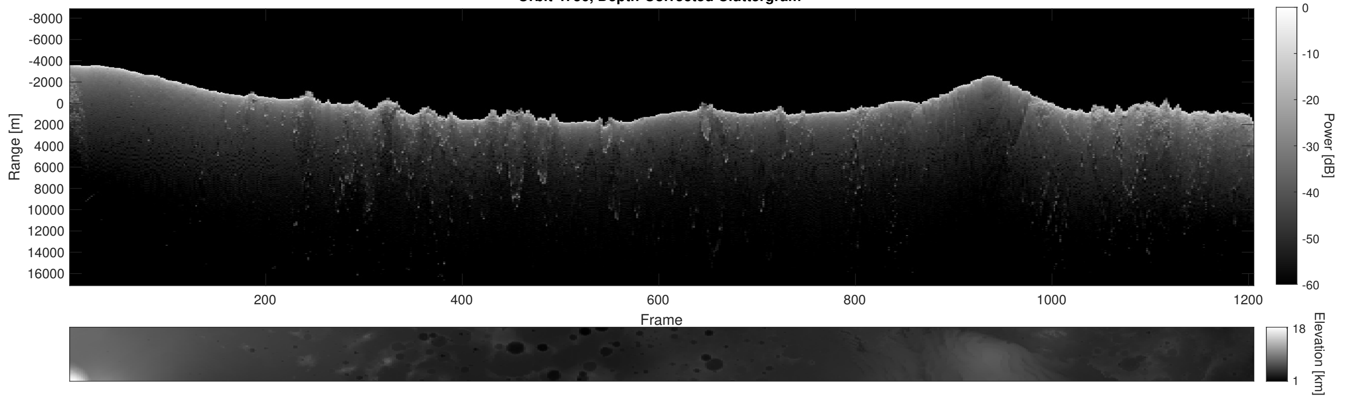
Orbit 4756, Depth-Corrected Cluttergram
