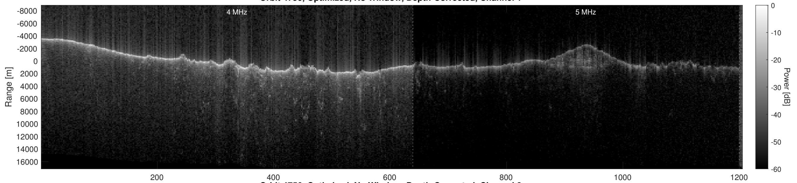
Orbit 4756, Optimized, No Window, Depth-Corrected, Channel 2
