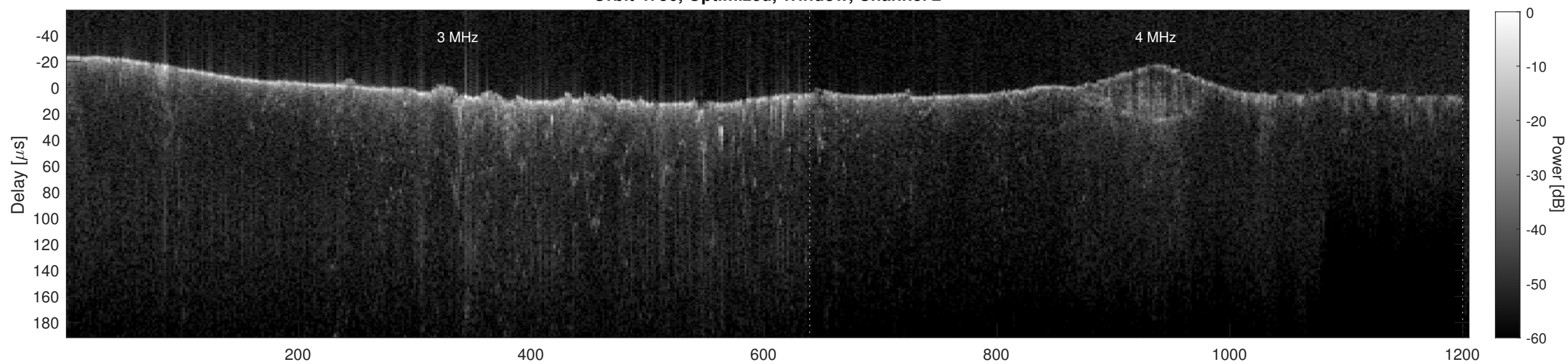
Orbit 4756, Cluttergram
