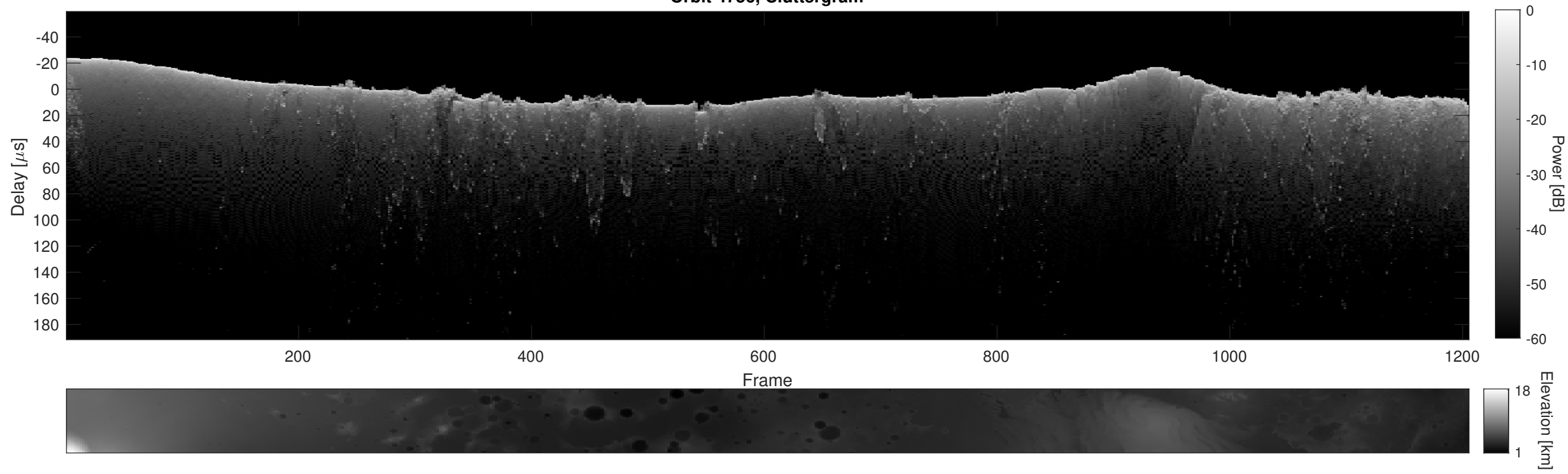
Orbit 4756, Cluttergram
