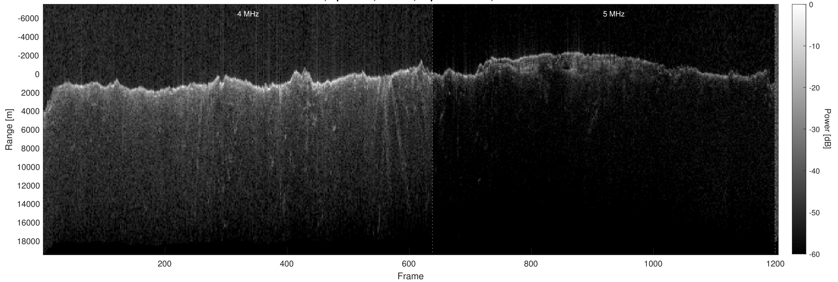
Orbit 4757, Optimized, Window, Depth-Corrected, Channel 2
