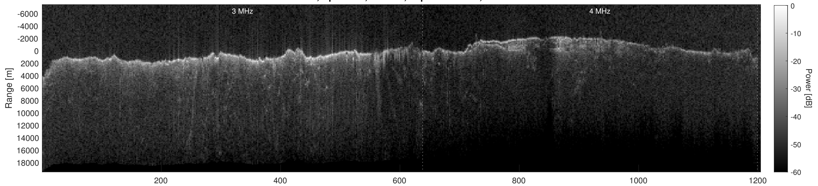
Orbit 4757, Depth-Corrected Cluttergram
