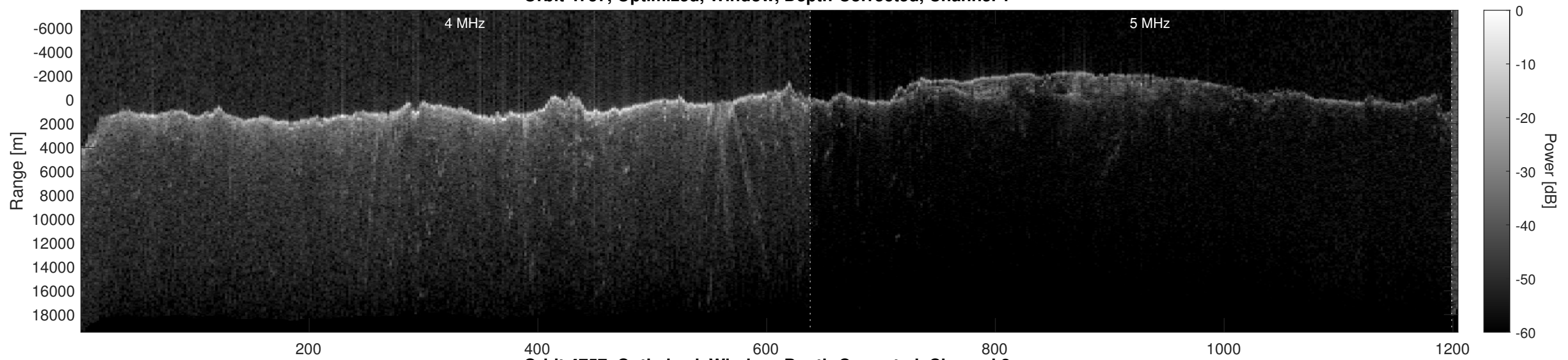
Orbit 4757, Optimized, Window, Depth-Corrected, Channel 2
