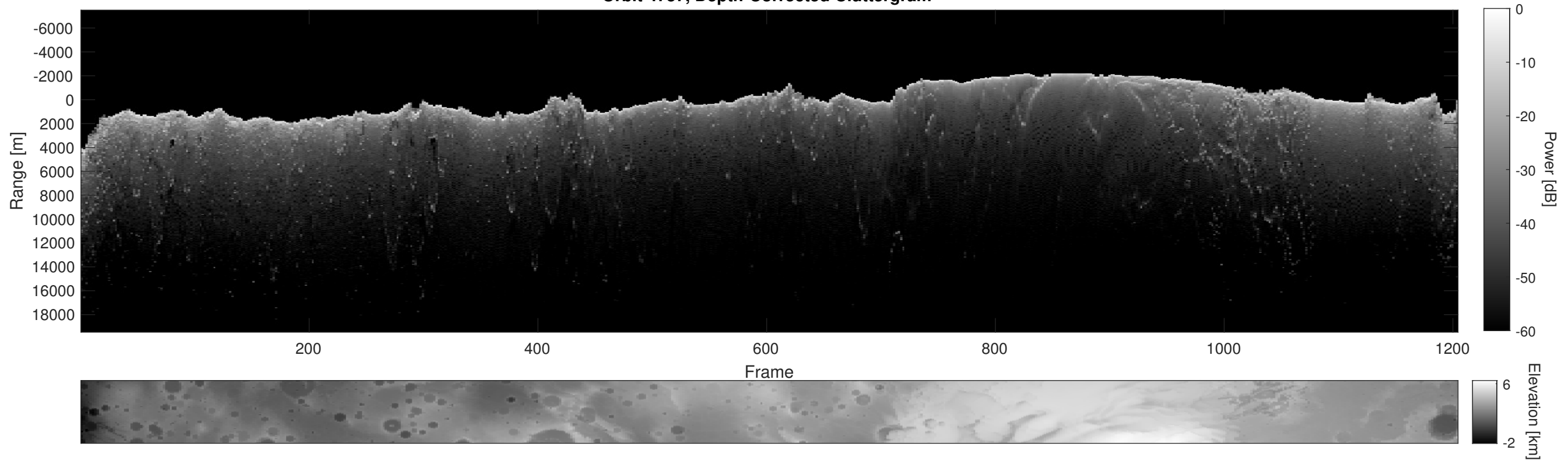
Orbit 4757, Depth-Corrected Cluttergram
