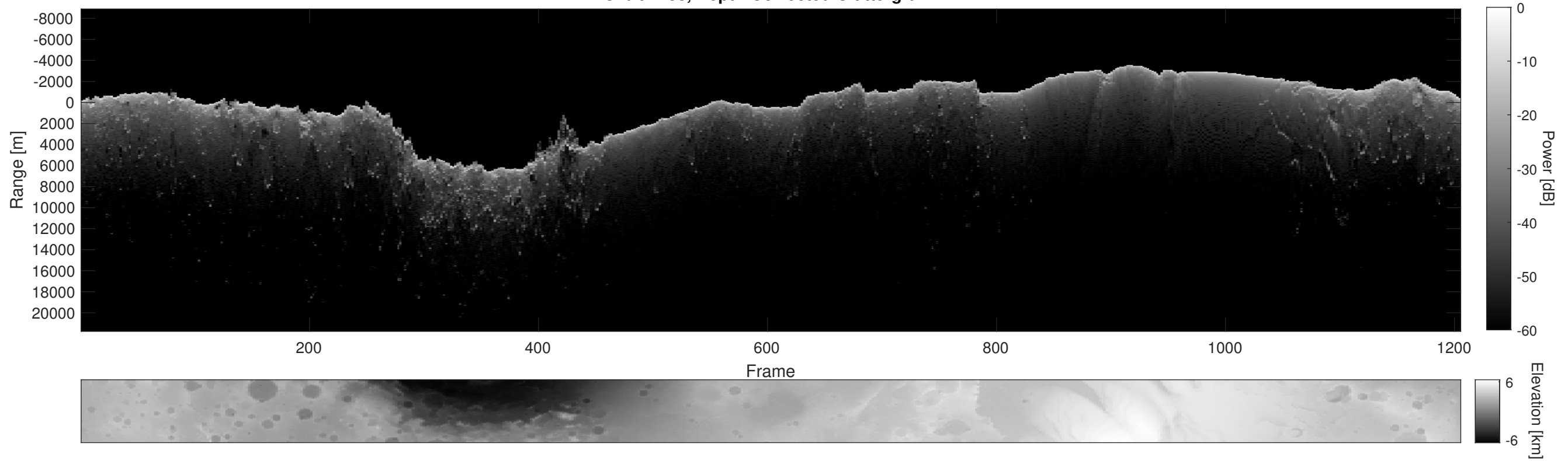
Orbit 4758, Depth-Corrected Cluttergram
