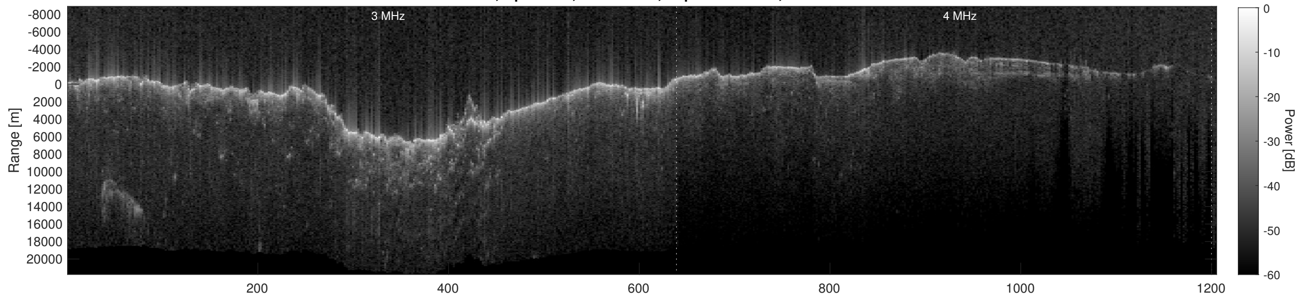
Orbit 4758, Depth-Corrected Cluttergram
