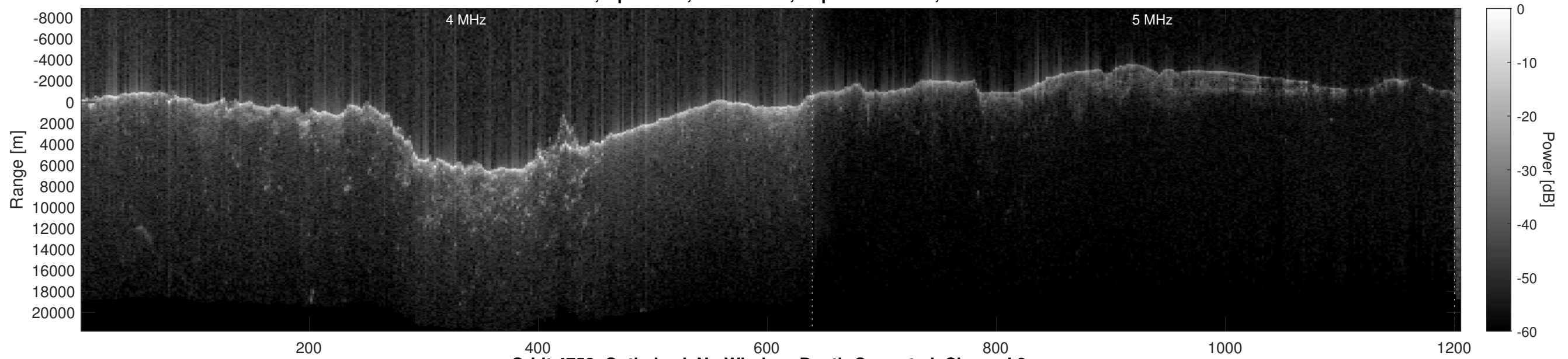
Orbit 4758, Optimized, No Window, Depth-Corrected, Channel 2
