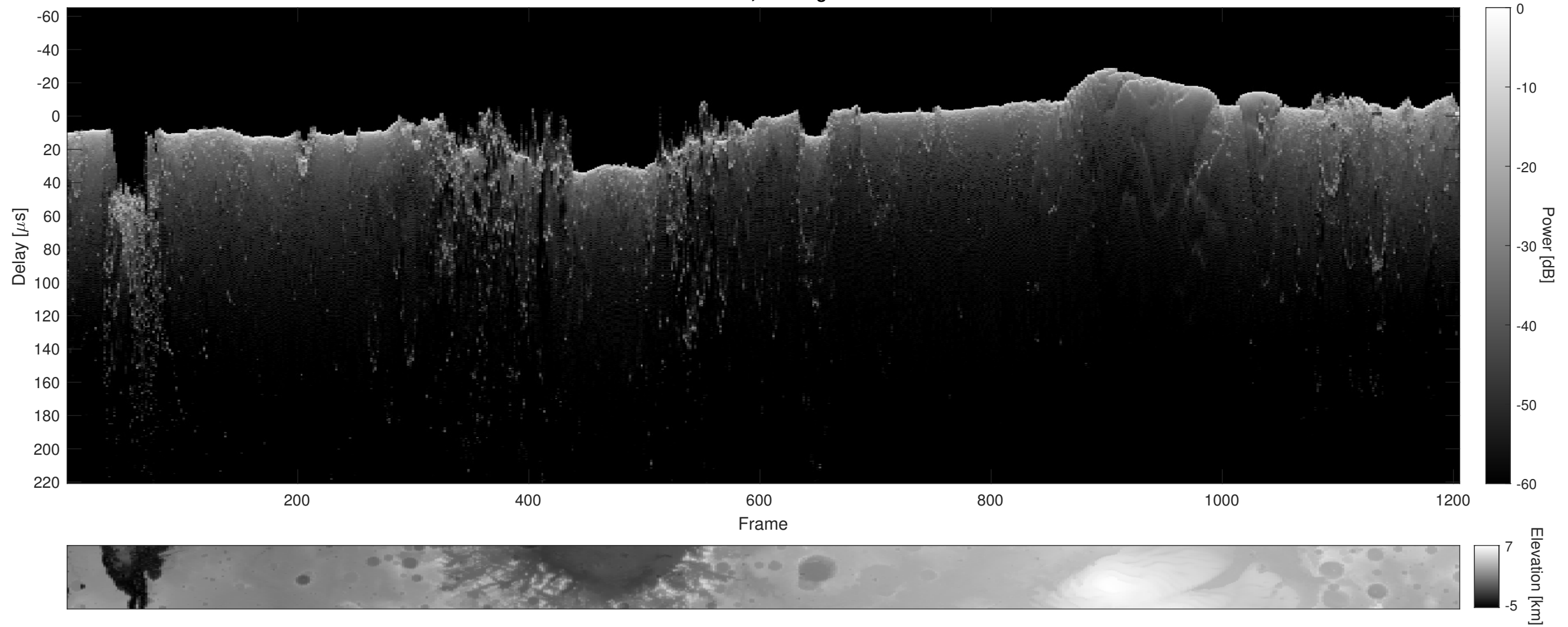
Orbit 4759, Cluttergram
