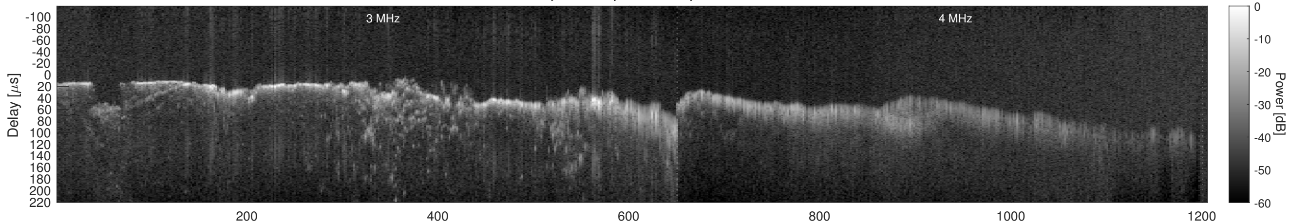
Orbit 4759, Window, Channel 2, Chapman
