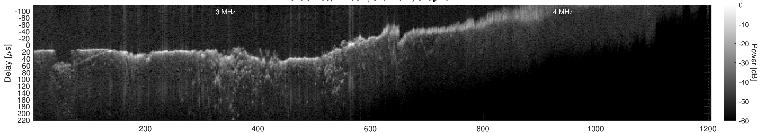
Orbit 4759, Window, Channel 2, Optimized
