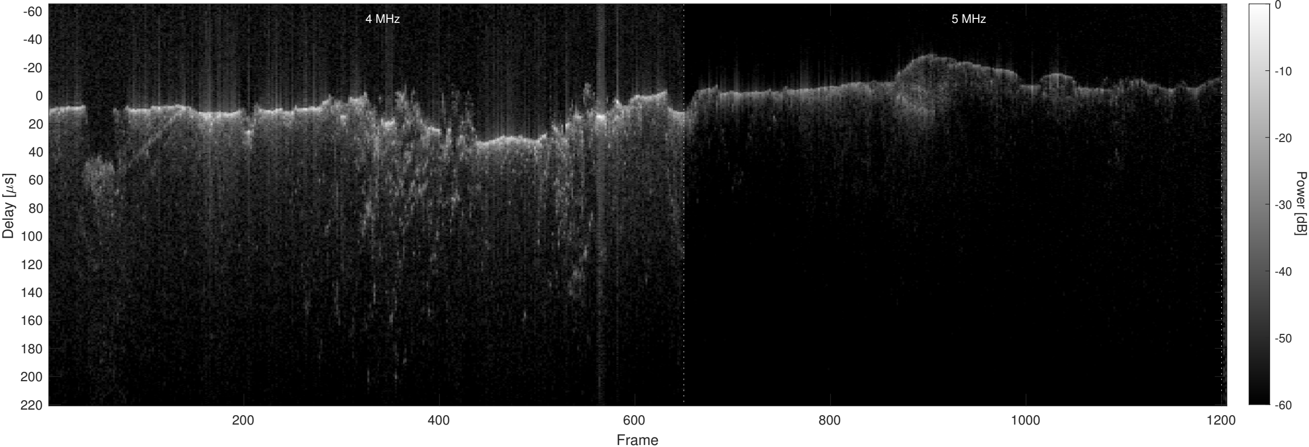
Orbit 4759, Optimized, No Window, Channel 2
