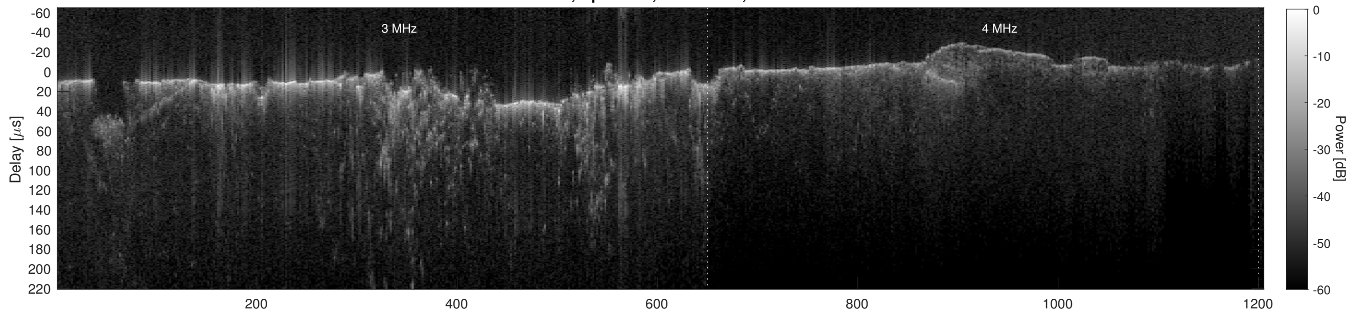
Orbit 4759, Cluttergram
