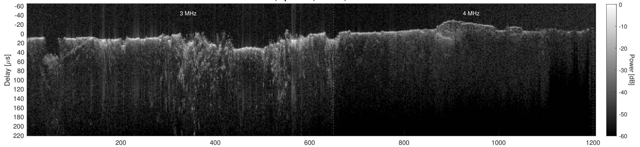
Orbit 4759, Cluttergram
