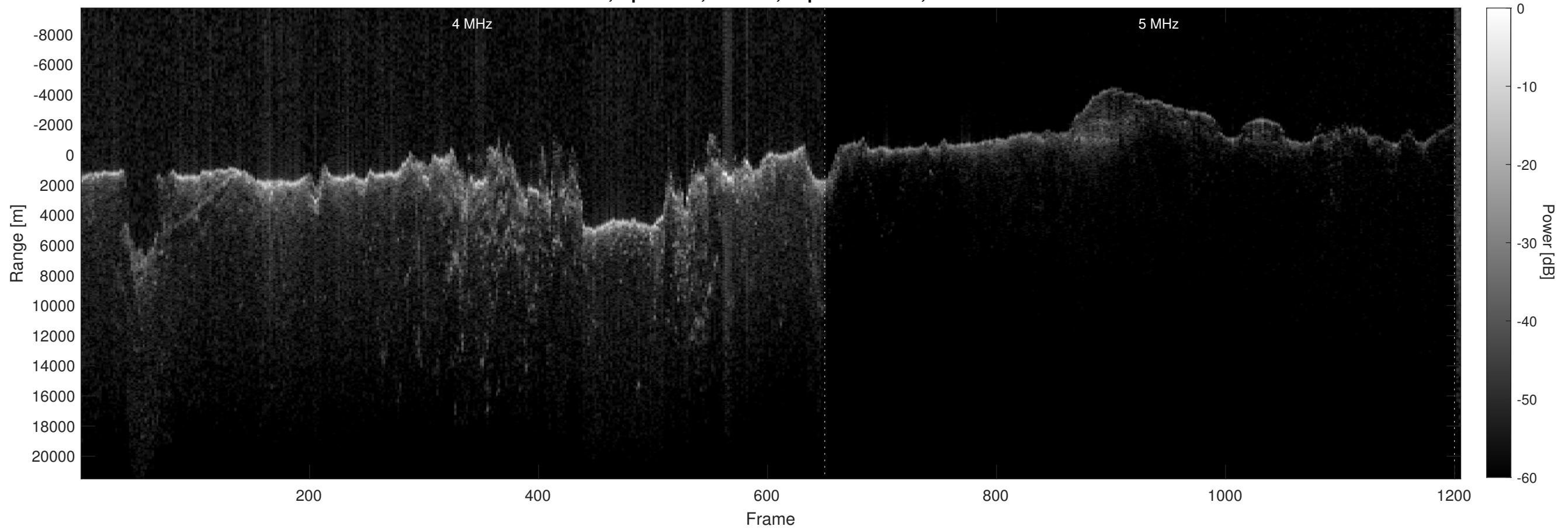
Orbit 4759, Optimized, Window, Depth-Corrected, Channel 2
