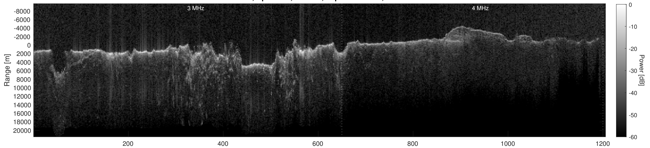
Orbit 4759, Depth-Corrected Cluttergram
