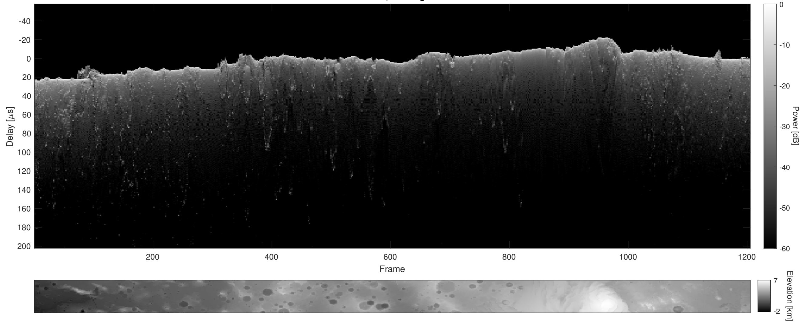
Orbit 4760, Cluttergram
