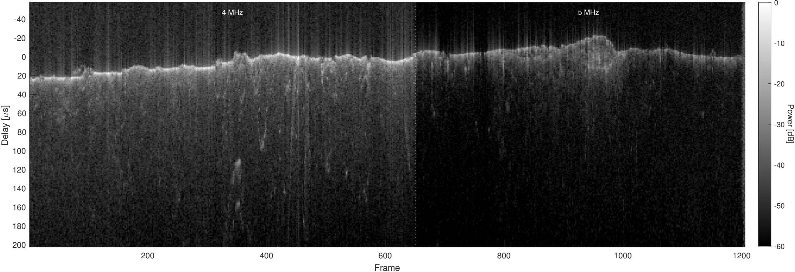
Orbit 4760, Optimized, No Window, Channel 2
