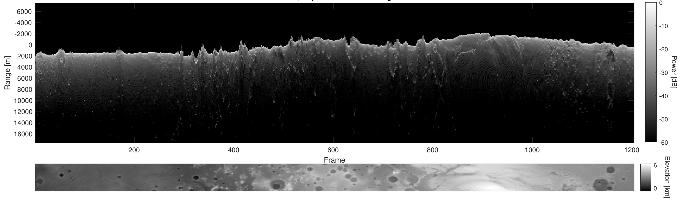
Orbit 4761, Depth-Corrected Cluttergram
