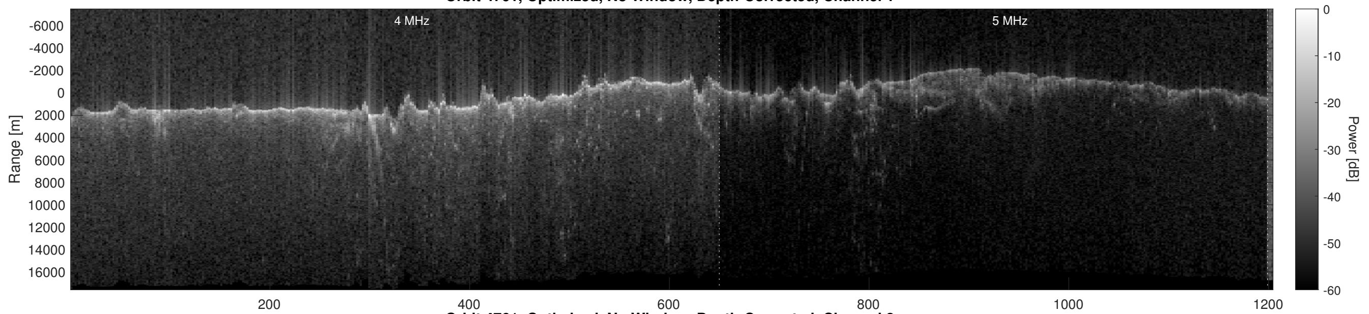
Orbit 4761, Optimized, No Window, Depth-Corrected, Channel 2
