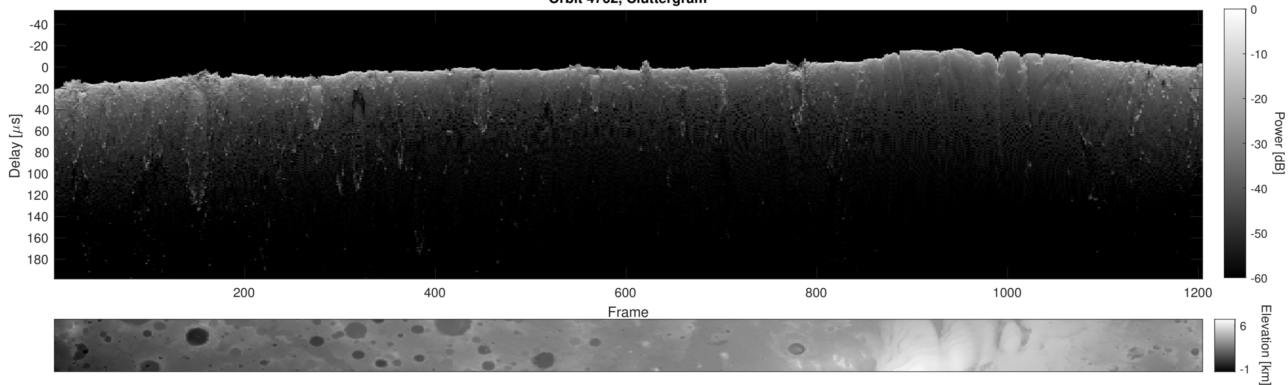
Orbit 4762, Cluttergram
