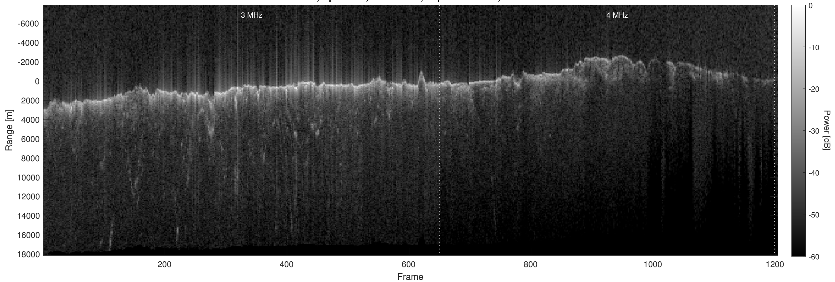
Orbit 4762, Optimized, No Window, Depth-Corrected, Channel 2
