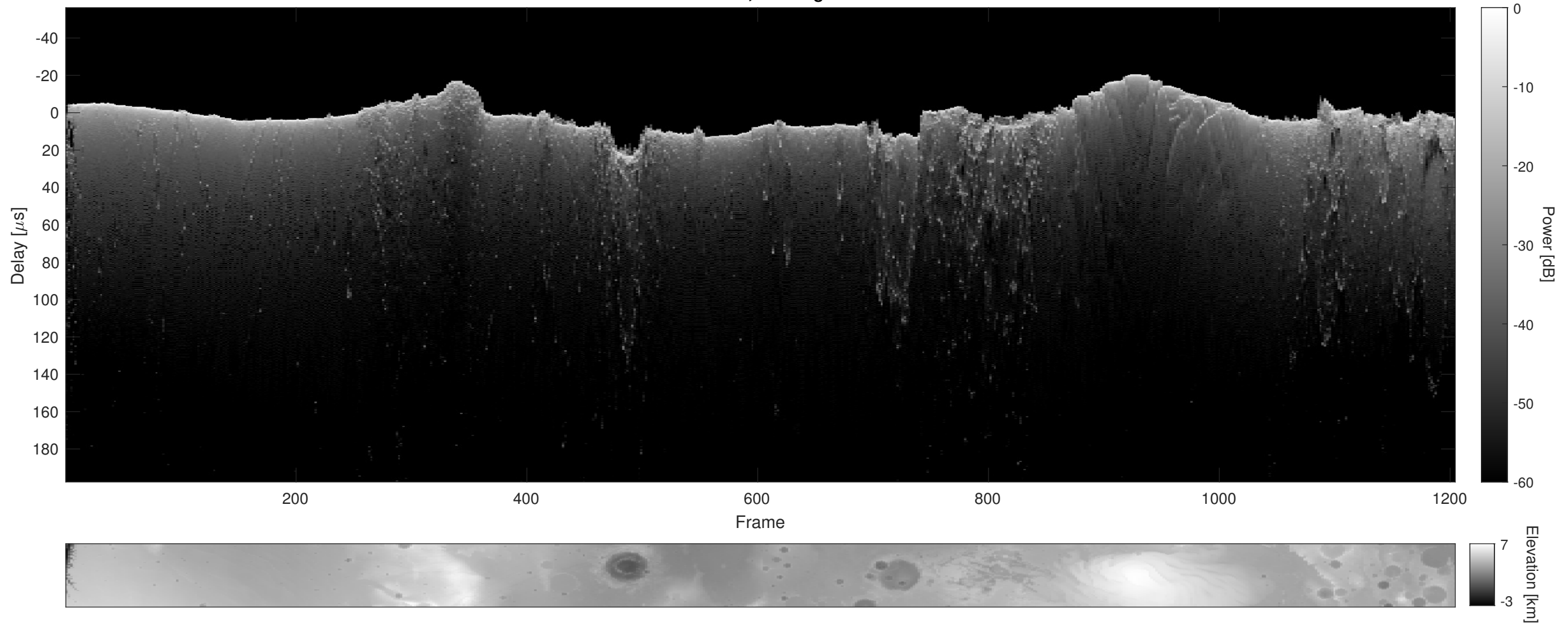
Orbit 4763, Cluttergram
