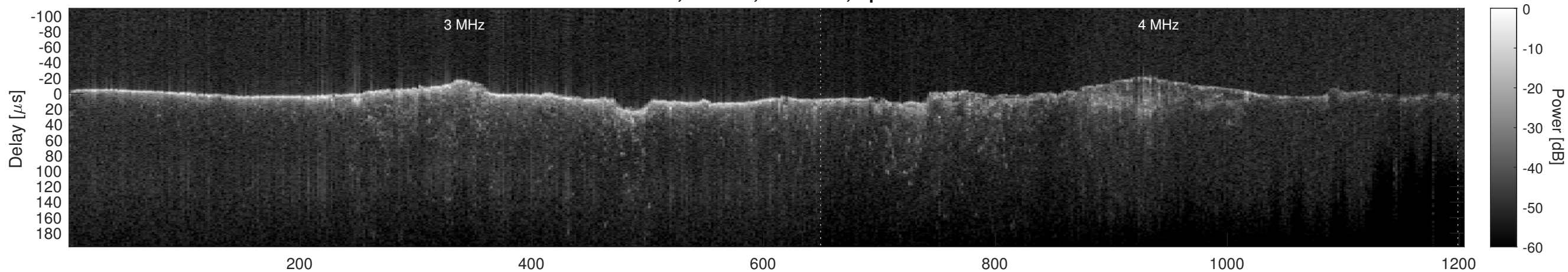
Orbit 4763, Cluttergram
