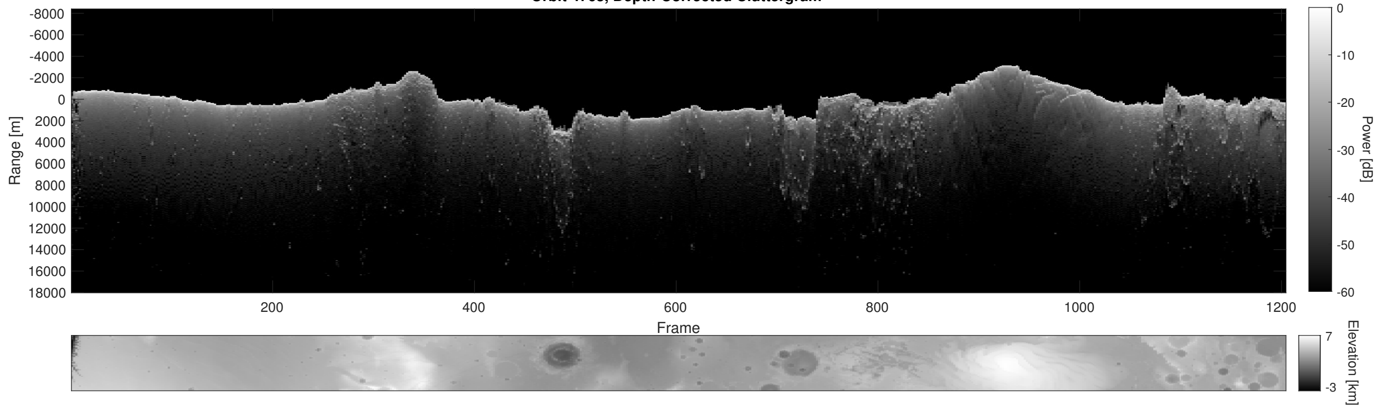
Orbit 4763, Depth-Corrected Cluttergram
