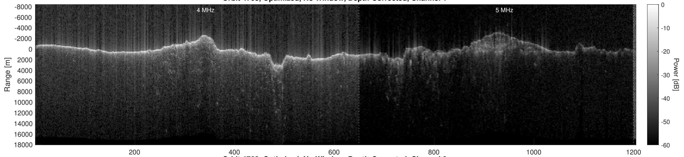
Orbit 4763, Optimized, No Window, Depth-Corrected, Channel 2
