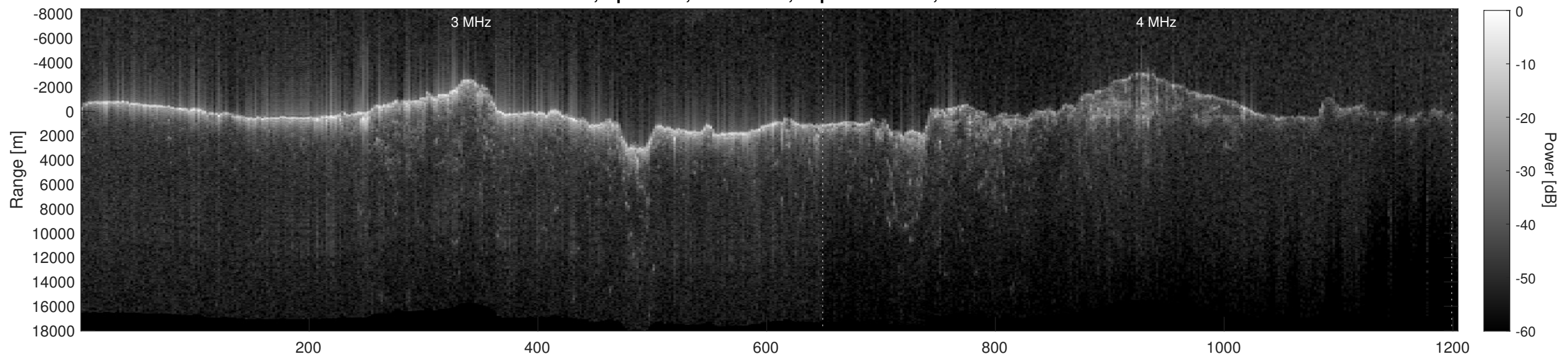
Orbit 4763, Depth-Corrected Cluttergram
