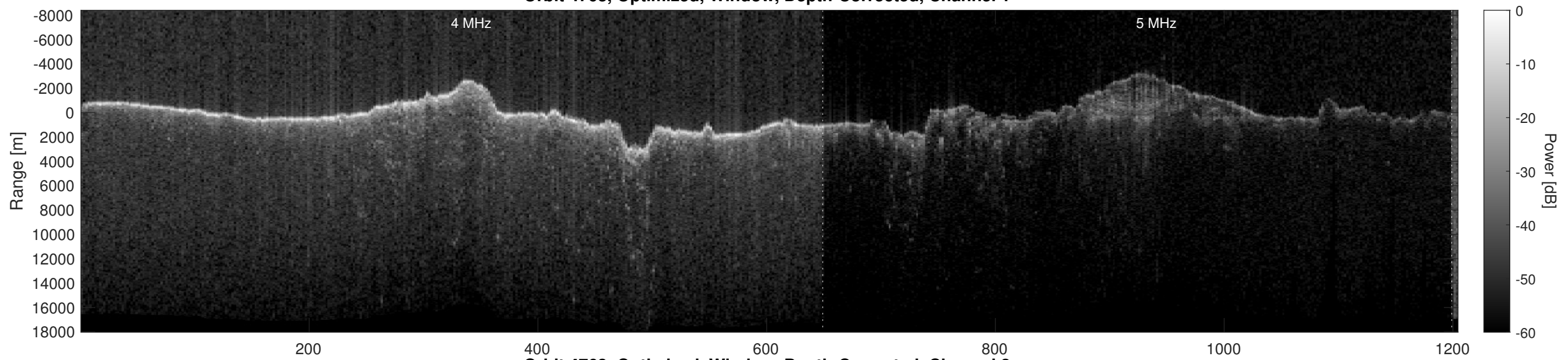
Orbit 4763, Optimized, Window, Depth-Corrected, Channel 2
