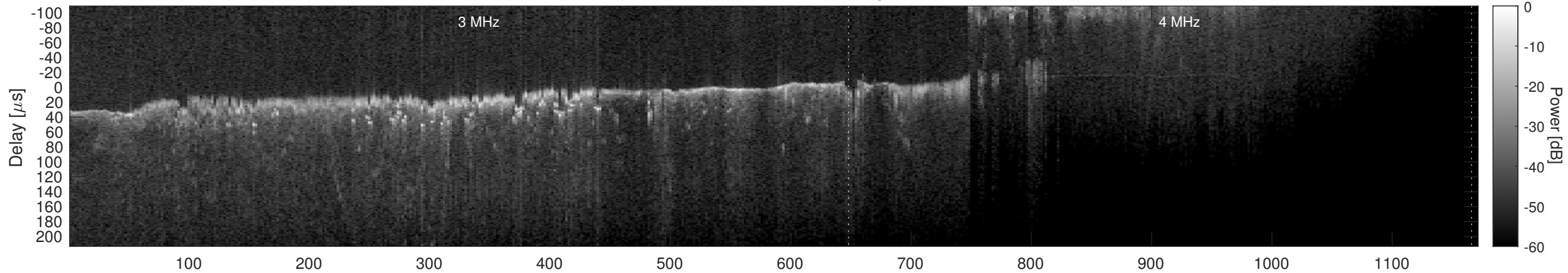
Orbit 4764, Cluttergram
