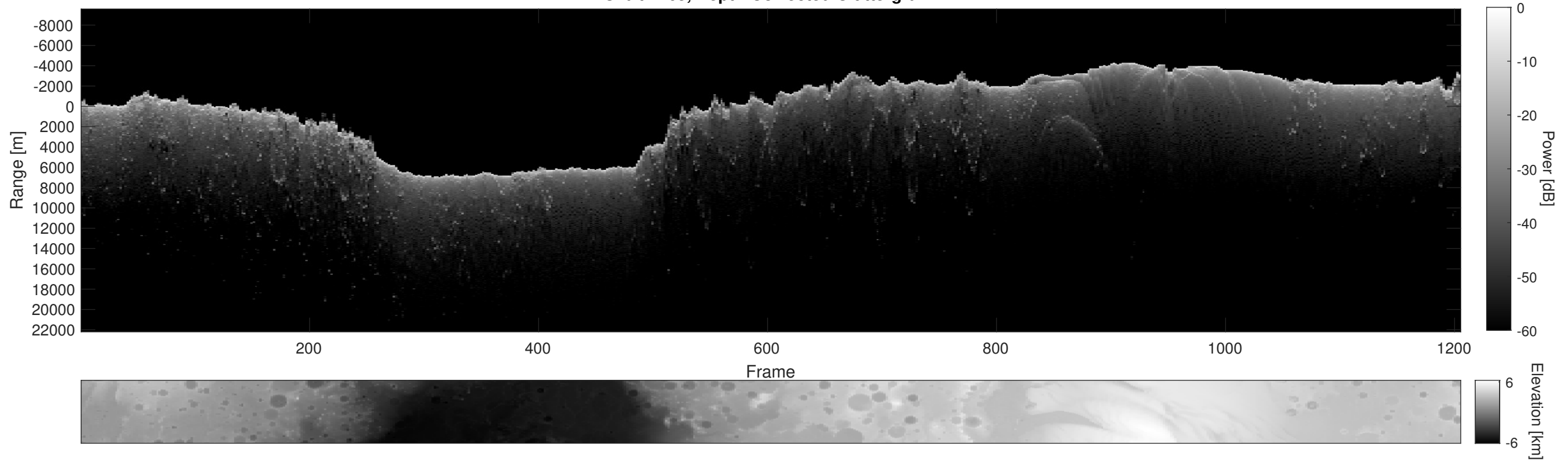
Orbit 4765, Depth-Corrected Cluttergram
