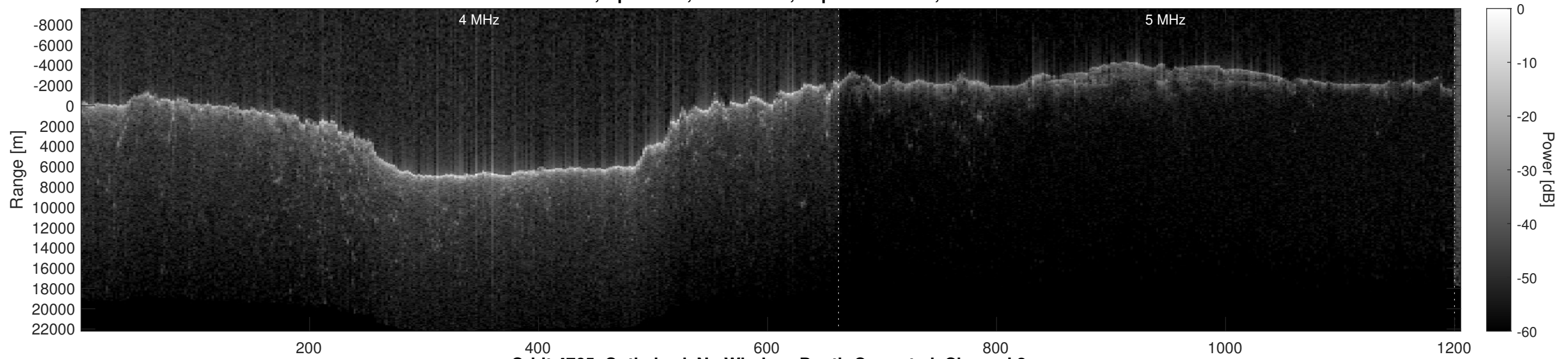
Orbit 4765, Optimized, No Window, Depth-Corrected, Channel 2
