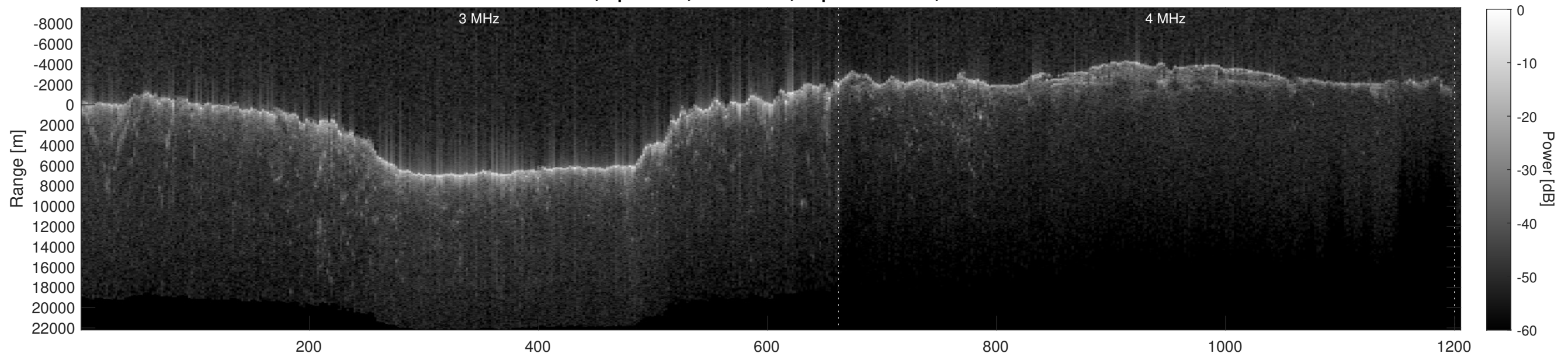
Orbit 4765, Depth-Corrected Cluttergram
