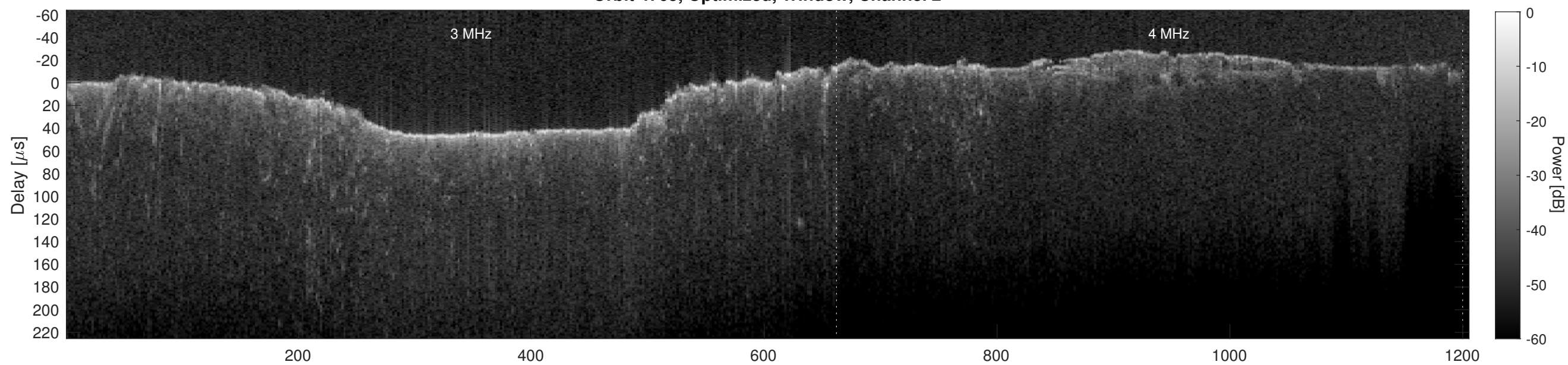
Orbit 4765, Cluttergram
