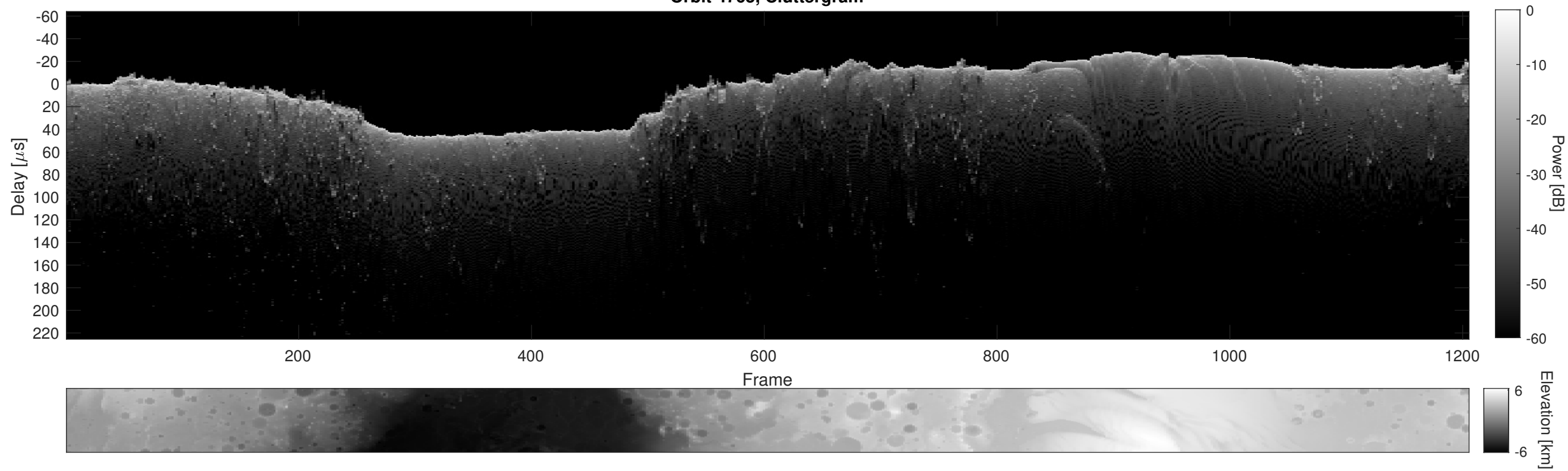
Orbit 4765, Cluttergram
