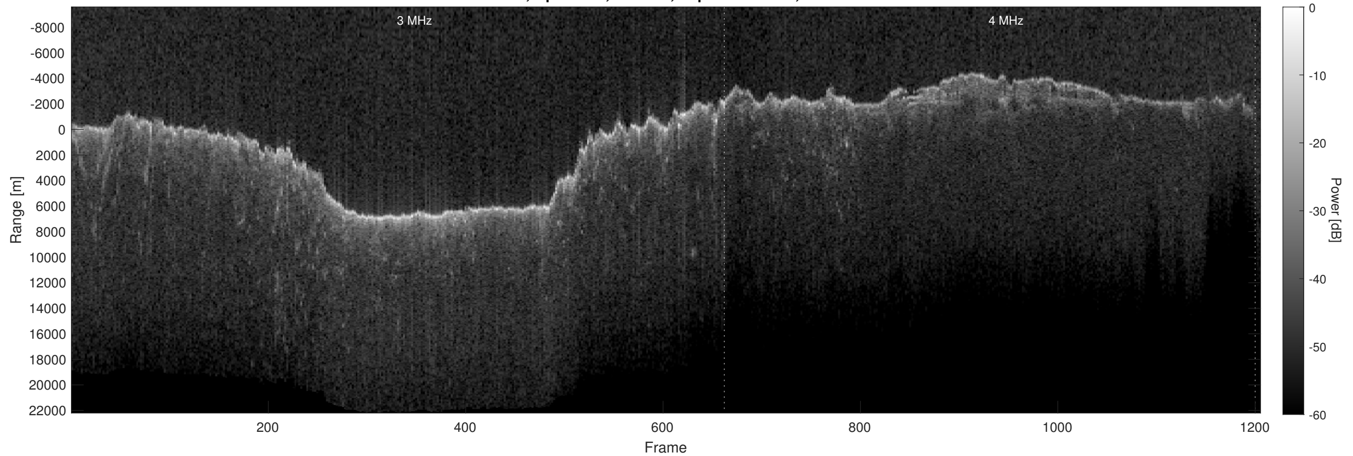
Orbit 4765, Optimized, Window, Depth-Corrected, Channel 2
