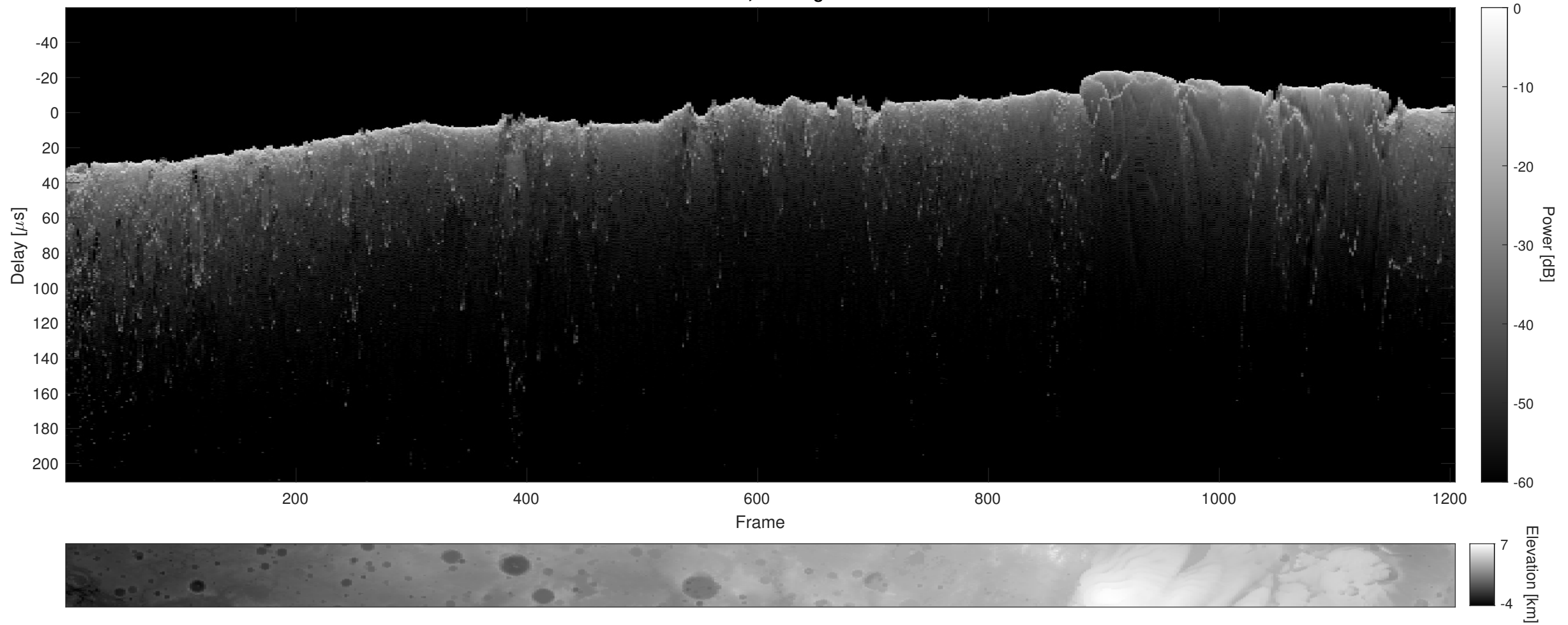
Orbit 4766, Cluttergram
