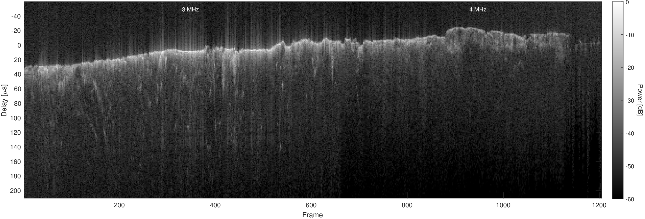
Orbit 4766, Optimized, No Window, Channel 2
