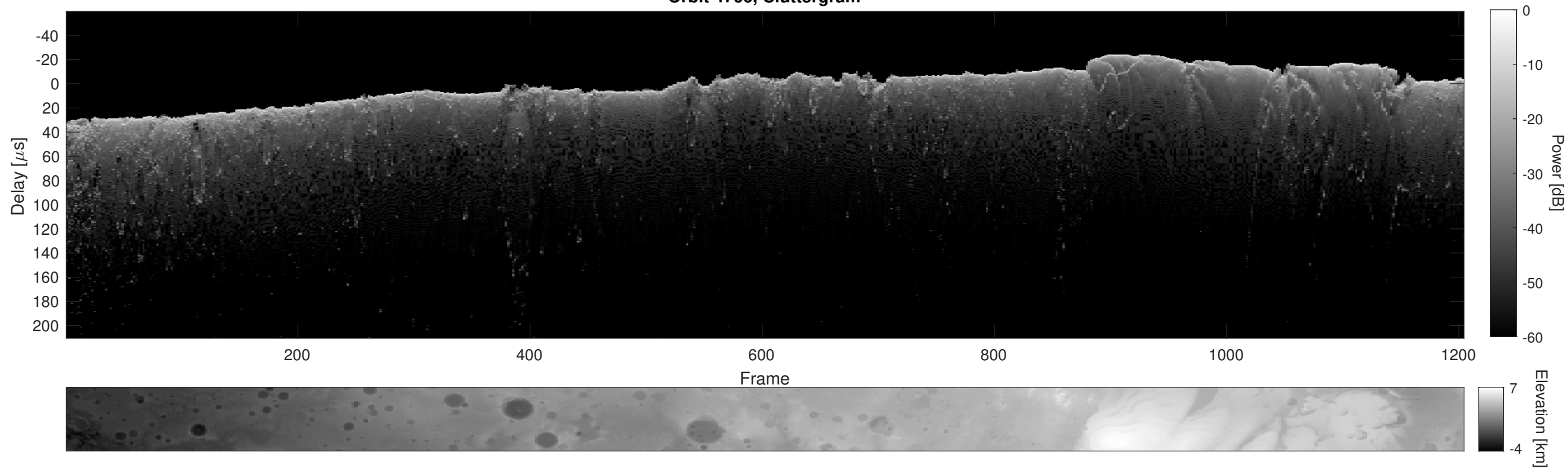
Orbit 4766, Cluttergram
