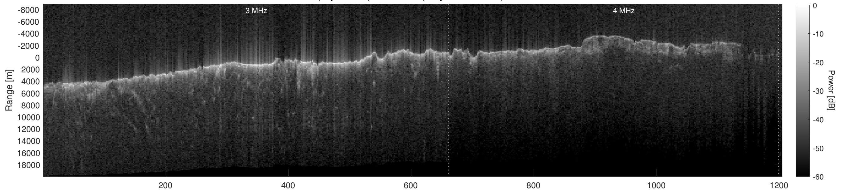
Orbit 4766, Depth-Corrected Cluttergram
