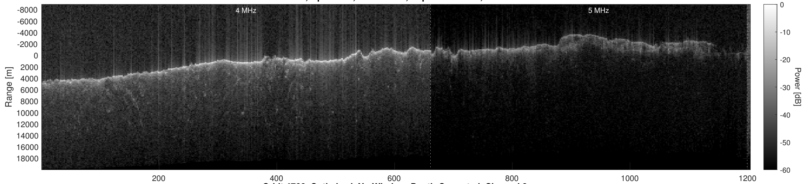
Orbit 4766, Optimized, No Window, Depth-Corrected, Channel 2
