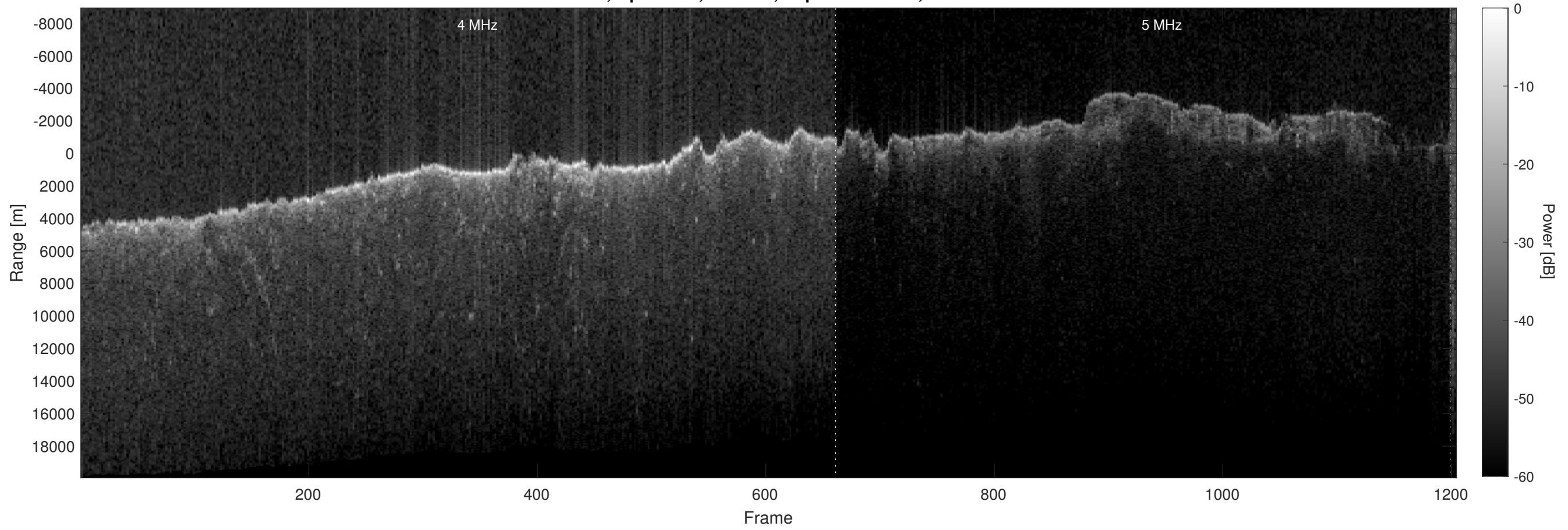
Orbit 4766, Optimized, Window, Depth-Corrected, Channel 2
