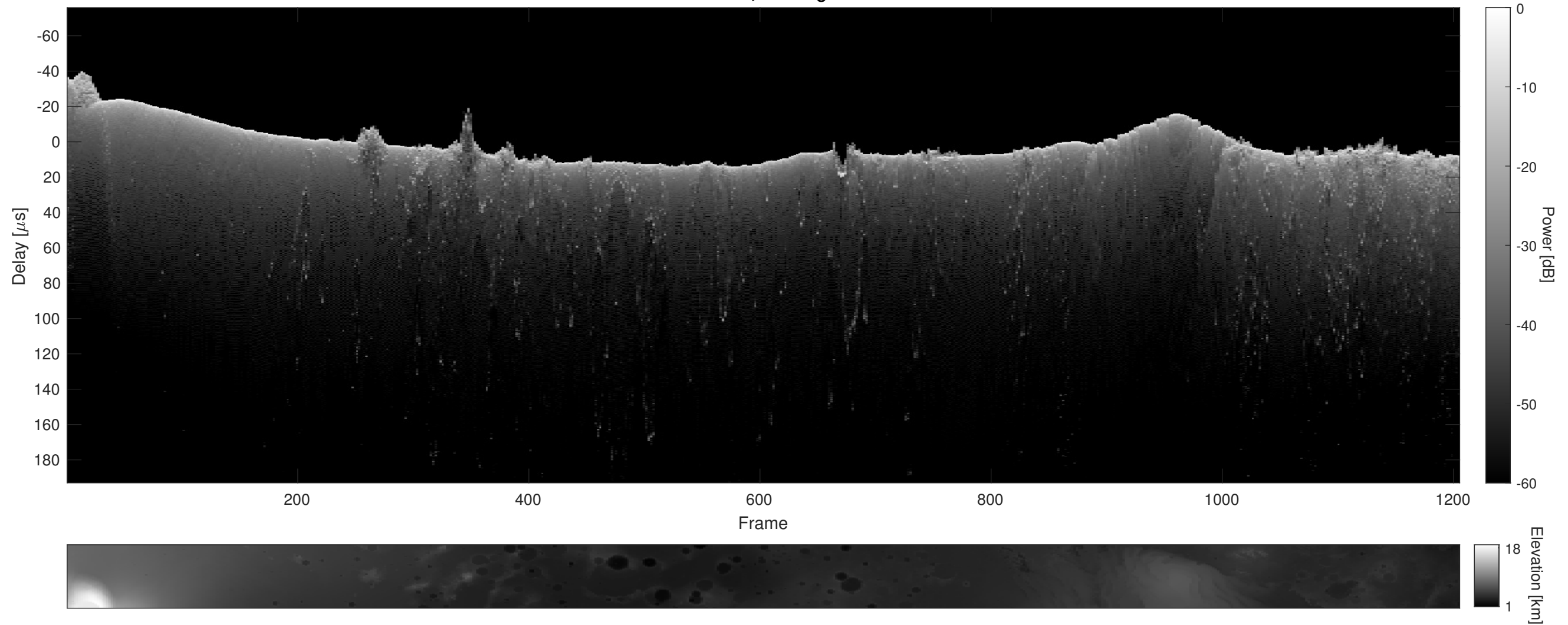
Orbit 4767, Cluttergram
