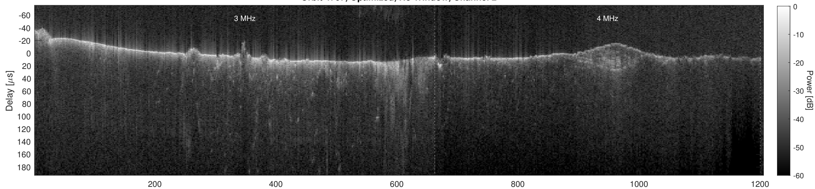
Orbit 4767, Cluttergram
